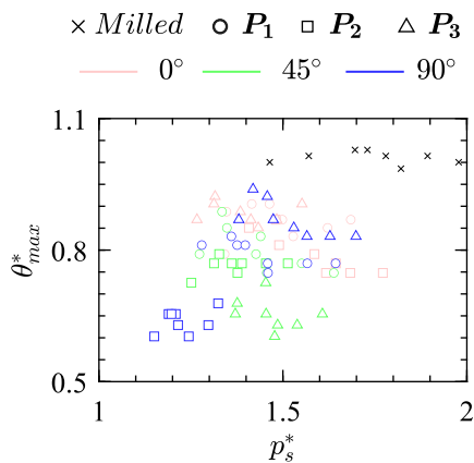
Fig. 7. Relationship between the non-dimensional required supply pressure p_s^* and the non-dimensional maximum jet deflection angle \theta_{max}^* . The respective raster angle and printer is indicated in the legend.
