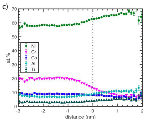
Fig. 4. (a) Cr distribution in a 5 nm thick slice of the metal. (b) Cr 15% isoconcentration surfaces. (c) a proxigram shows the Ni, Cr, Co, Al, and Ti content as a function of the distance to the isoconcentration surfaces in (b).
