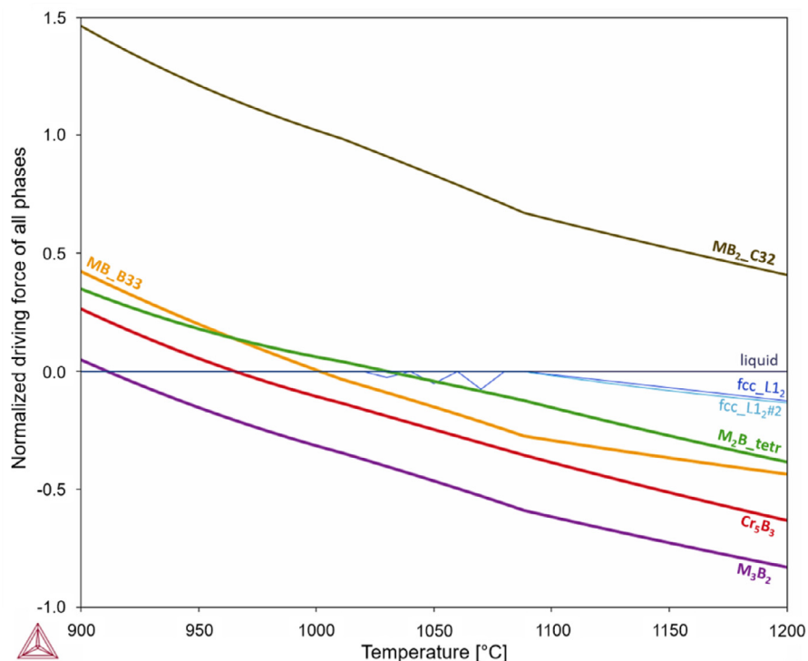
Fig. 9. Thermodynamic prediction of boride formation in IN738LC with formation from the liquid for positive driving forces (with MB_2 as most stable boride) and formation from the solid state for negative driving forces (with M_2B , MB , and M_5B_3 as stable borides).
