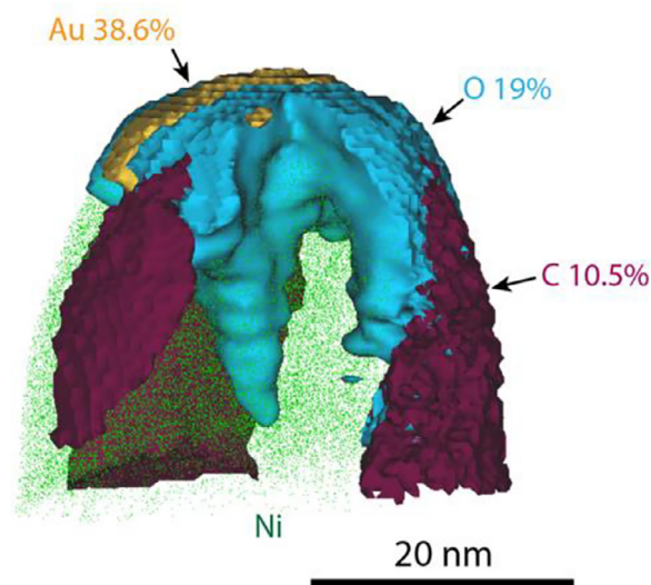
Fig. 5. Reconstruction of APT analysis. Isoconcentration surfaces corresponding to Au 38.6% (yellow), O 19% (blue) and C 10.5% (burgundy) are shown as well as a small part of the Ni atoms in the metal matrix. The values of the isoconcentration surfaces are set to visualize the different volumes in the best way. Three carbides, all cutting the edge of the analysis, are sitting in the oxide specimen surface.
