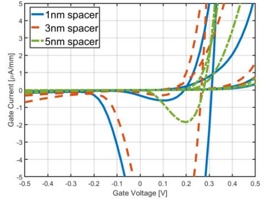
Fig. 5. Gate current of the 100 nm gate-length InP HEMT with spacer thickness of 1 nm (blue solid), 3 nm (red dashed) and 5 nm (green dash-dot) at 5 K. V_{DS} = 0.1 - 0.9 V in steps of 0.2 V.
