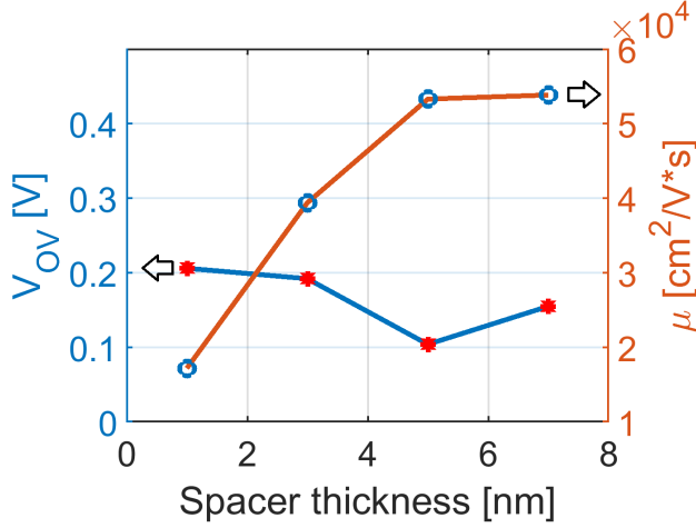
Figure 3.15: The V_{OV} at optimum noise gate bias and \mu for the InP HEMT versus d_{sp} at 5 K.
