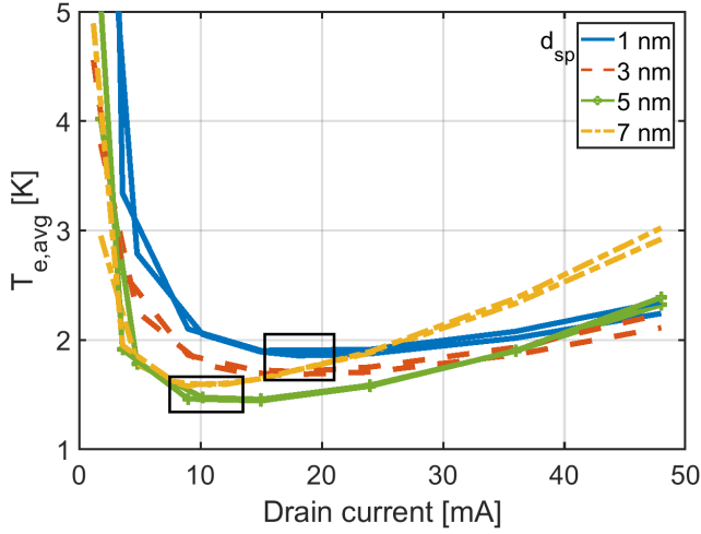
Figure 3.10: The T_{e,avg} for InP HEMT LNAs with d_{sp} = 1 (blue), 3 (red), 5 (green) and 7 nm (yellow) versus I_D at 5 K and the drain biases of V_{ds}=0.325 V and 0.475 V. Black boxes indicate the minimum noise regions.
