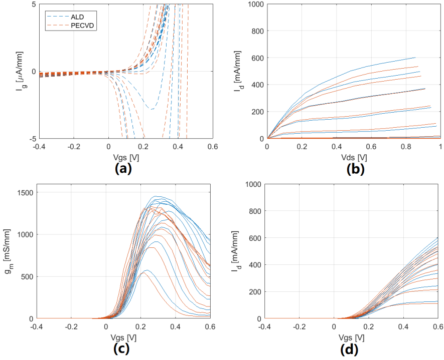
Figure 2.8: dc characterization of 4 x 50 μm InP HEMTs at 300 K using passivation of PECVD Si x N y (red) and ALD Al 2 O 3 (blue) with a plasma cleaning process. (a) Gate current versus gate voltage, with drain voltage 0 - 1 V in steps of 0.1 V. (b) Drain current versus drain voltage, with gate voltage -0.4 - 0.6 V in steps of 0.1 V. (c) Transconductance versus gate voltage, with drain voltage 0 - 1 V in steps of 0.1 V. (d) Drain current versus gate voltage, with drain voltage 0 - 1 V in steps of 0.1 V.
