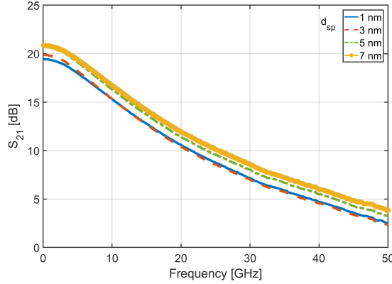
Figure 3.8: The S_{21} measurements at 5 K of the InP HEMT with d_{sp} = 1 (blue), 3 (red), 5 (green) and 7 nm (yellow) all at the bias points of I_d = 5 mA and V_{ds} = 0.475 V.
