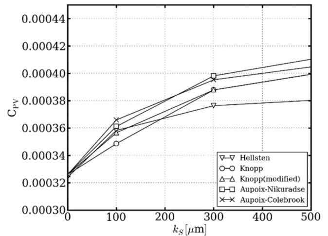
Fig. 22. C_{PV} for KCS at Re = 2.89 \times 10^9 , EASM, k_S range 0–500 \mu\text{m} .
