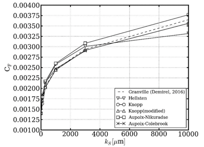
Fig. 18. Roughness model comparison for a flat plate at Re = 2.89 \times 10^9 , k-\omega SST, k_s range 0–10 000 \mu\text{m} .
