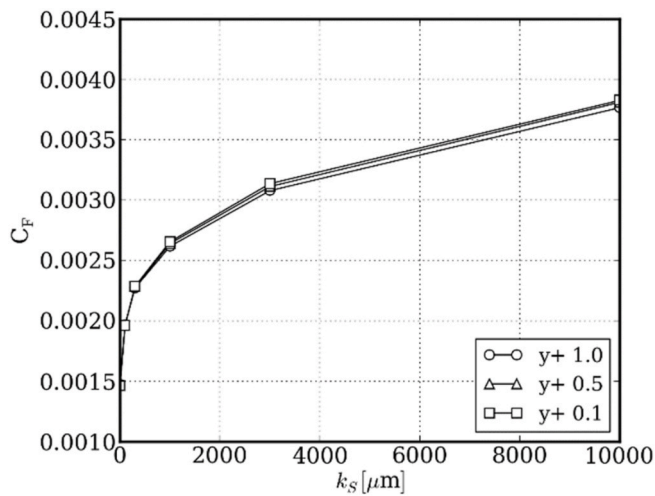
Fig. 11. Influence of y^+ on C_F , k-\omega SST, Aupoix-Colebrook, range 0–10 000 \mu\text{m} .
