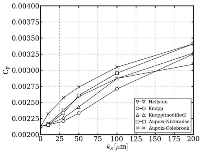
Fig. 16. Frictional resistance coefficient at Re = 7.6 \times 10^7 , EASM.
