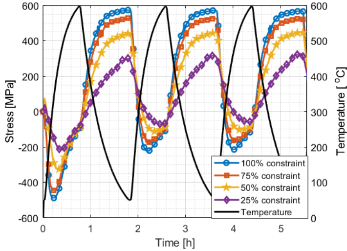
Figure 3.3: Stress and temperature for the thermomechanical experiments with a maximum temperature of 650 °C.
