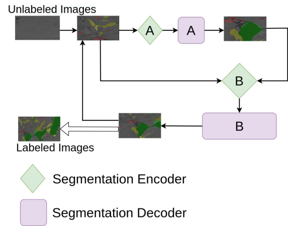
Fig. 1. Architecture of the CSSA method.
