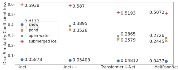
Fig. 4. Comparison of segmentation performance in terms of DSC loss (1-DSC/100) (the lower the better).
