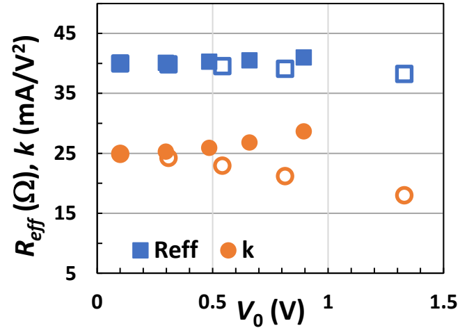
Fig. 2. Effective resistances and transconductance parameters extracted for the five residual voltages using data from gate voltages -3.5 , -3 , -1 V (open symbols) and from -3.5 , -3 , 0 V (filled symbols).
