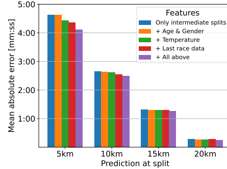
Fig. 2. Mean absolute error for neural network models with and without additional features
