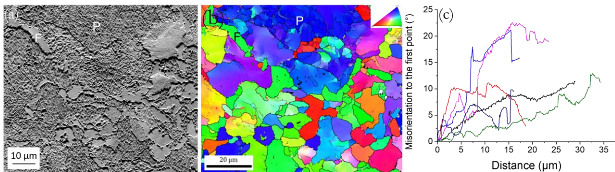
Figure 6. Microstructure and orientations in the sample annealed at 650 °C for 4 h. (a) SEM image, (b) IPF map, and (c) misorientation gradients within 6 randomly chosen pearlite grains. The colors in (b) represent the crystallographic orientation along the measured surface normal direction, see inset.
