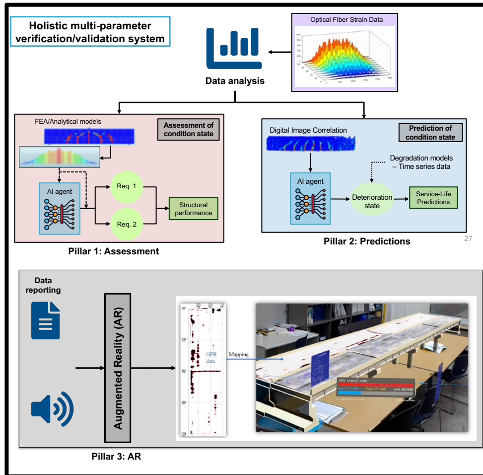
Figure 4. A proposal for a conceptual system architecture consisting of three pillars: Pillar 1 – Assessment, Pillar 2 – Predictions and Pillar 3 – Augmented Reality
