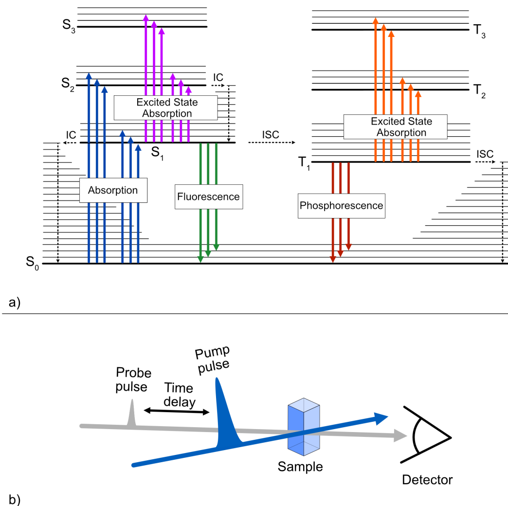
Figure 3.2: a) Modified Jablonski diagram which includes excited state absorption (ESA) for the singlet and triplet excited states. Photoexcitation and radiative decay are marked as solid lines and non-radiative processes are marked as dotted lines. b) Schematic illustration of TA showing how a sample is photoexcited by a pump pulse and then subsequently interrogated by a probe pulse after some time delay.
