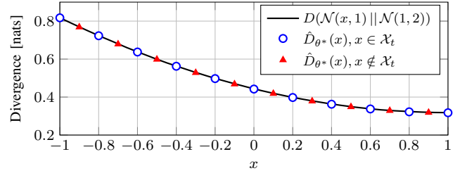
Fig. 1: Accuracy and generalization ability of the trained divergence estimator (6), where \mathcal{X}_t = \{-1, -0.8, \dots, +1\} .
