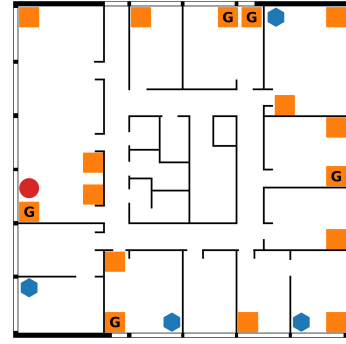
Fig. 2: Local testbed of 500\text{ m}^2 . Red circle: synchronization node; Orange squares: Nodes equipped with our GPIO tracing system ( Grace ); Blue hexagons: other nodes; Marker G: nodes equipped with GPS.
