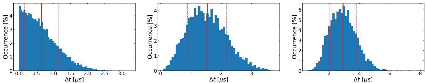
(a) Occurrences of offsets between two radio receivers. Avg: 0.65 \mu\text{s} , Std: 487 ns.
