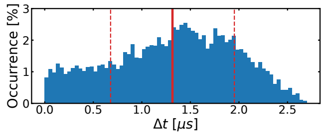
(b) Offset distribution of a radio's input signal from the radio output signal of the synchronization node. Avg offset (solid red line): 1.32 \mu\text{s} , Std (dashed red lines): 637 ns.
