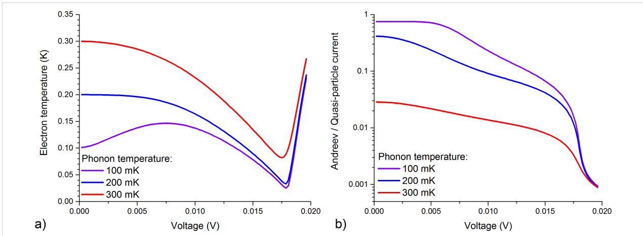
Figure 2: (a) The electron temperature of the absorber determined from the solution of the heat balance equation for sample OL-G7nn; (b) the ratio between Andreev current and quasi-particle current at phonon temperatures of 300, 200, and 100 mK for the same sample.
