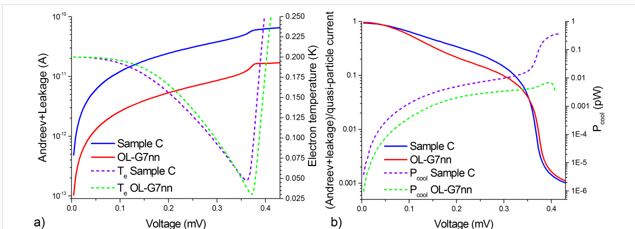
Figure 3: (a) The sum of the Andreev and leakage currents found by solving the heat balance equation for samples C from [7] and OL-G7nn (left axis, solid curves) at 200 mK phonon temperature, recalculated to a single bolometer in the array, and the electron temperatures for samples C and OL-G7nn (right axis, dashed curves); (b) the ratio between the sum of the Andreev and leakage currents and the quasi-particle current of two samples (left axis, solid curves), recalculated to a single bolometer in the array, and the cooling powers for samples C and OL-G7nn (right axis, dashed curves).
