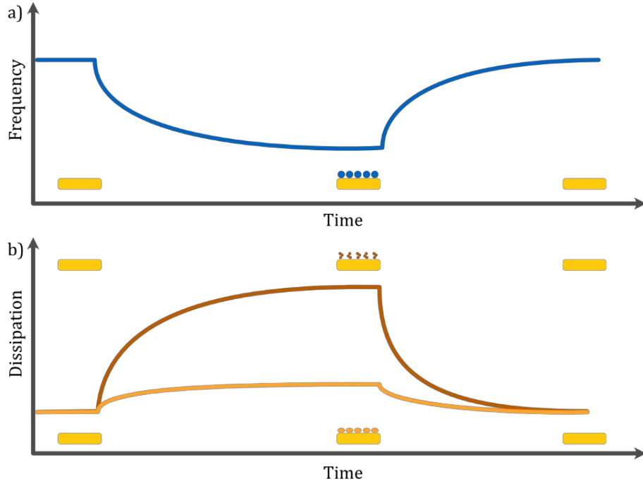
Figure 8. QCM-D configuration (a) frequency change as a function of time, as molecules adsorb or desorb from the surface and (b) dissipation response of soft (brown) and rigid (yellow) layer deposition and immigration from surface
