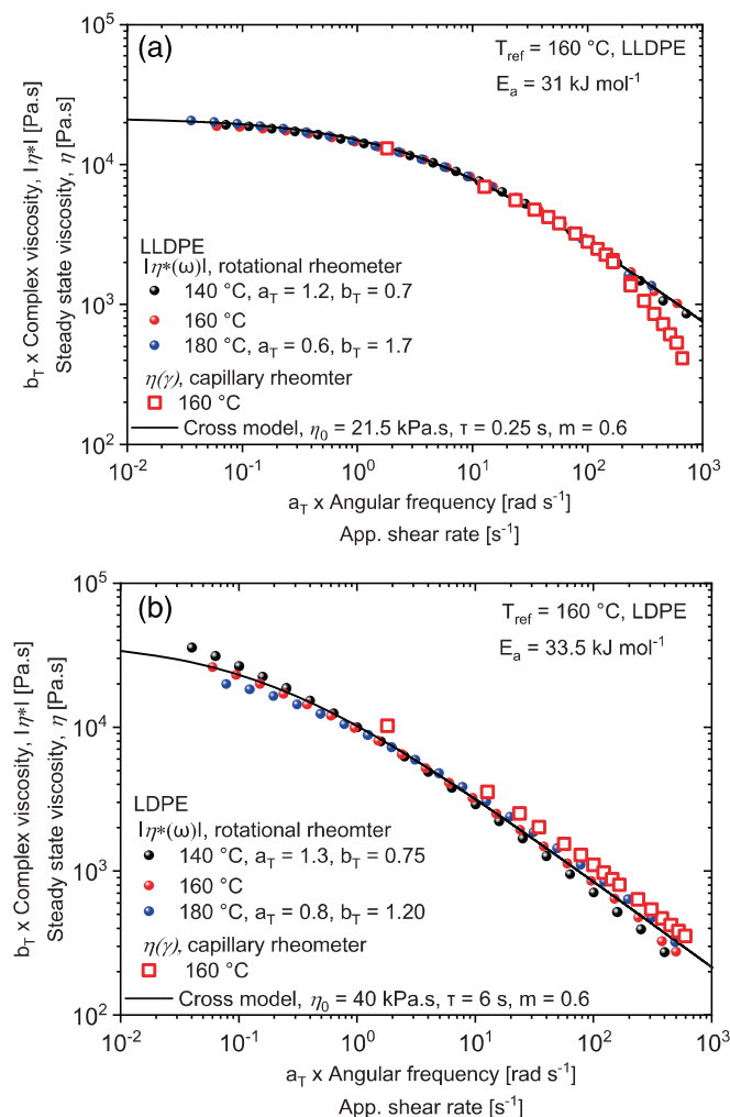
FIGURE 7 Master curve of the magnitude of the complex viscosity as a function of angular frequency at reference temperature of T = 160^\circ\text{C} for (a) LLDPE and (b) LDPE. Steady-state viscosity as a function of apparent shear rate obtained at T = 160^\circ\text{C} as well. the experimental results of the magnitude of complex viscosity are fitted by cross model (Equation (1)). [Color figure can be viewed at wileyonlinelibrary.com ]
