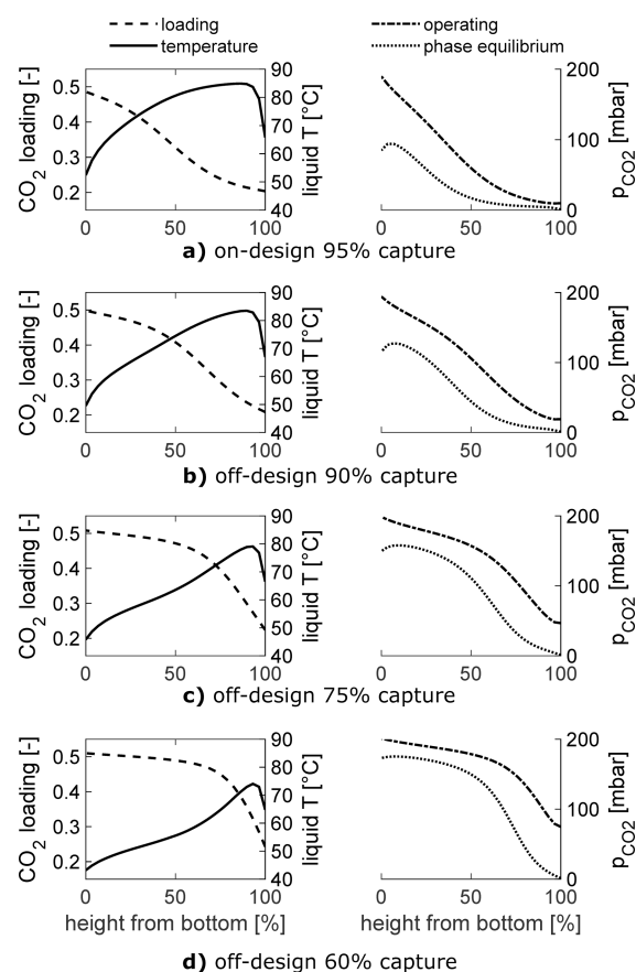
Figure 10. Absorber profiles for liquid temperature and molar CO 2 loading (left panels) and McCabe-Thiele plots of the partial CO 2 pressure (right panels) depending on the capture rate (rows a–d) for a fixed absorber design (height of 20 m, design factor of 80 and 95% capture) and a CO 2 concentration of 20 vol % wet . Plots are obtained from the model simulations performed in this work.
