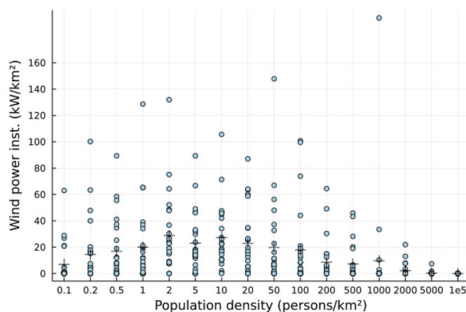
Fig. 4. Wind deployment in relation to population density for the 25 analyzed regions. The black crosses indicate averages across all regions, and the blue circles show capacities in specific regions.
