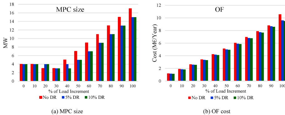
Fig. 12. The impact of DR on MPC size and OF cost based on load increment with N-1 in MG1.
