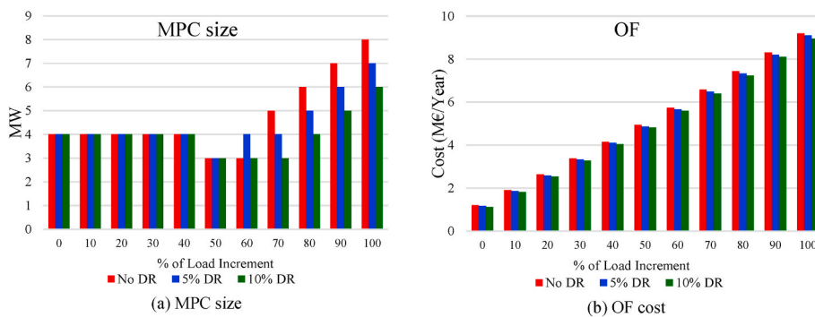
Fig. 13. The impact of DR on MPC size and OF cost based on load increment with N-1 in MG2.
