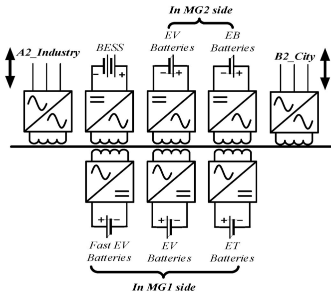
Fig. 7. Topology of the proposed MPC for the case study.
