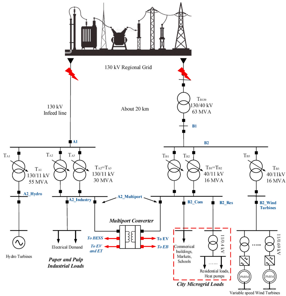
Fig. 14. Single line diagram of case study for island mode investigation.
