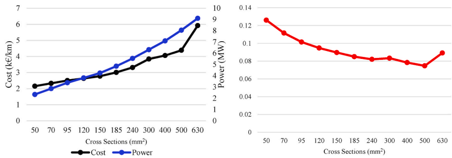
Fig. 10. The techno-economic curves for the different cross sections of cables.
