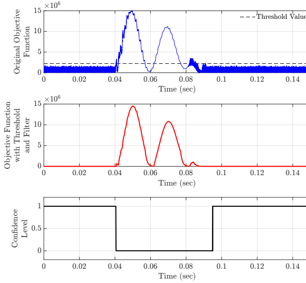
Figure 5.6: MATLAB Simulink results in terms of the original objective function, objective function with threshold and filter, and confidence level for a three-phase fault with resistive load.
