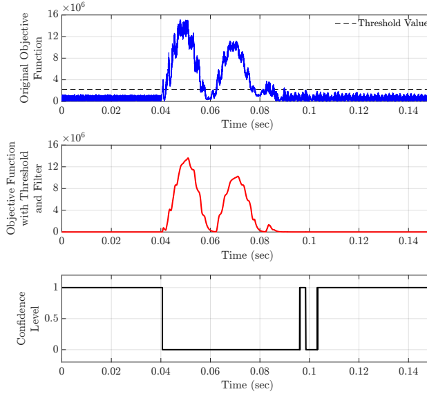
Figure 5.9: MATLAB Simulink results in terms of the original objective function, objective function with threshold and filter, and confidence level for a three-phase fault with R-L load of pf 0.8.
