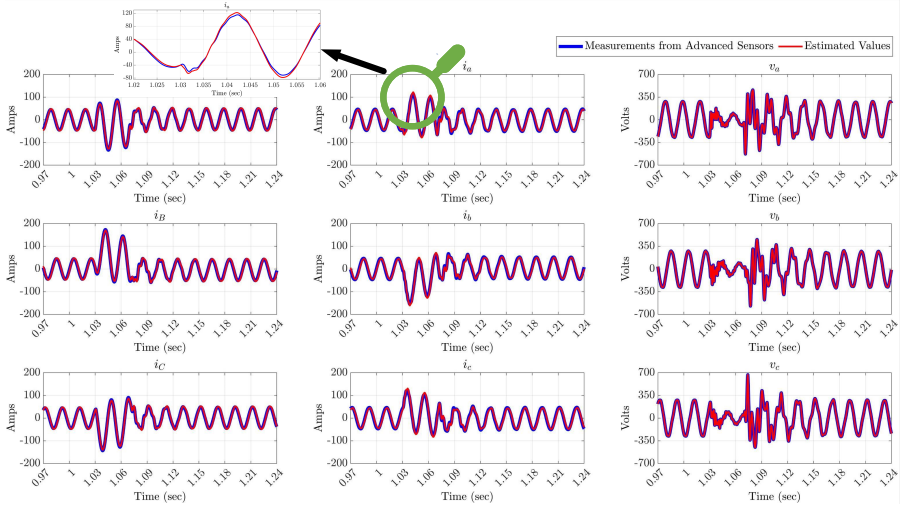
Figure 6.24: Validation results for a three-phase fault current fed from both ends in terms of measured and estimated values of the sending end currents ( i_a , i_b , i_c ), receiving end currents ( i_a , i_b , i_c ), and receiving end voltages ( v_a , v_b , v_c ).
