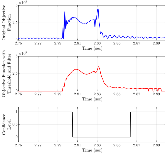
Figure 6.10: Validation results for a three-phase fault with resistive load in terms of objective function and confidence level.
