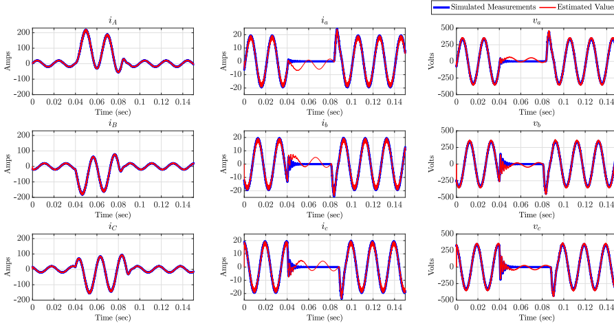
Figure 5.5: MATLAB Simulink results in terms of simulated measurements and their estimated values of the sending end currents ( i_A , i_B , i_C ), receiving end currents ( i_a , i_b , i_c ), and receiving end voltages ( v_a , v_b , v_c ) for a three-phase fault with resistive load.
