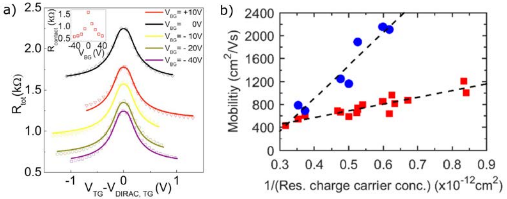
Figure 4.2: a) R_{\text{tot}} vs V_{\text{TG}} - V_{\text{Dirac,TG}} at selected V_{\text{BG}} values (symbols) along with modeling results for each data set (lines). The inset shows the extracted contact resistance R_{\text{contact}} vs V_{\text{BG}} . (Fig. from Ref. [73]. First published by Seyoung Kim, et al. "Realization of a high mobility dual-gated graphene field-effect transistor with \text{Al}_2\text{O}_3 dielectric", Appl. Phys. Lett. 94, 062107 (2009); https://doi.org/10.1063/1.3077021 ). b) "Low-field \mu of holes in GFETs found by fitting the drain-source resistance model ( \mu_{\text{R}} , Eq. (S1), squares) and using delay time analysis ( \mu_0 , circles) vs the inverse of the residual charge carrier concentration n_0 . Dashed lines are polynomial fitting curves and serve as guide for the eye. (Fig. from Supplementary of Ref. [52]. First published by Bonmann, M. et al., "Charge carrier velocity in graphene field-effect transistors", Appl. Phys. Lett. 111, 233505 (2017), doi: https://doi.org/10.1063/1.5003684 . Reprinted with CC BY 4.0-permission.)
