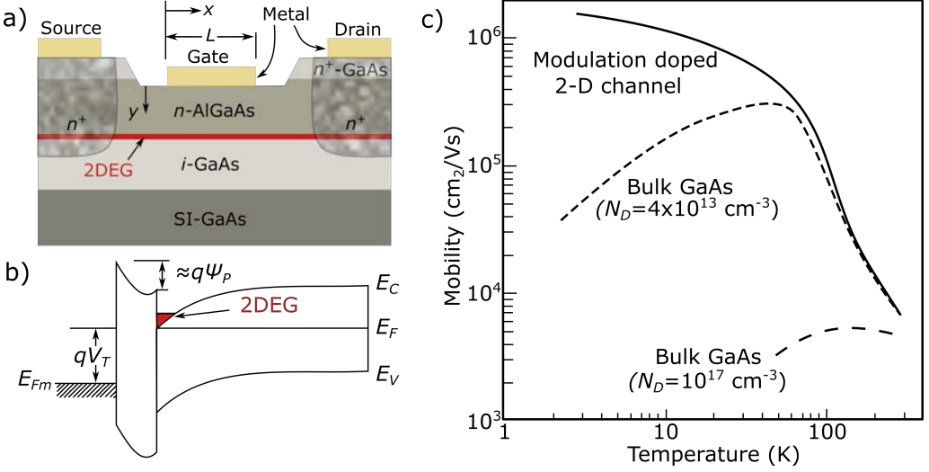
Figure 2.1: a) Typical structure of an HEMT, using the basic AlGaAs/GaAs system. b) Energy-band diagrams for an enhancement-mode HEMT at onset of threshold. c) Comparison of low-field electron mobility of modulation-doped 2-D channel to bulk GaAs at different doping levels. (Modified Fig. from Ref. [14], p.402-403)
