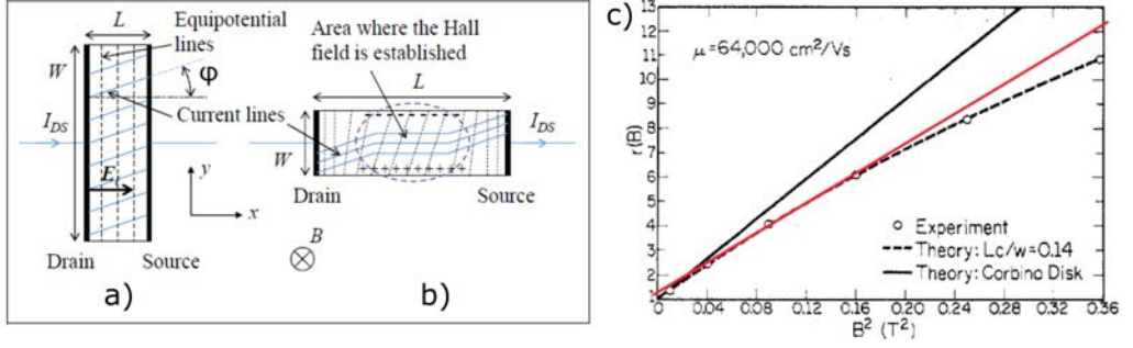
Figure 5.1: a) short transistor, b) long transistor, under B . [From Ref. [85]]. c) The reduced resistance r(B) = \frac{R(B)}{R(0)} for a structure with 100 \text{ } \mu\text{m} channel width and 14 \text{ } \mu\text{m} channel length as a function of B -field along with the calculated r(B) for electrons with a mobility of 64\,000 \text{ cm}^2/\text{Vs} . The measurement was made with no sample illumination at 77 \text{ K} in an electric field less than 1 \text{ V/cm} . Also shown is the r(B) relation for the Corbino disk geometry with the same mobility. [From Ref. [76]]
