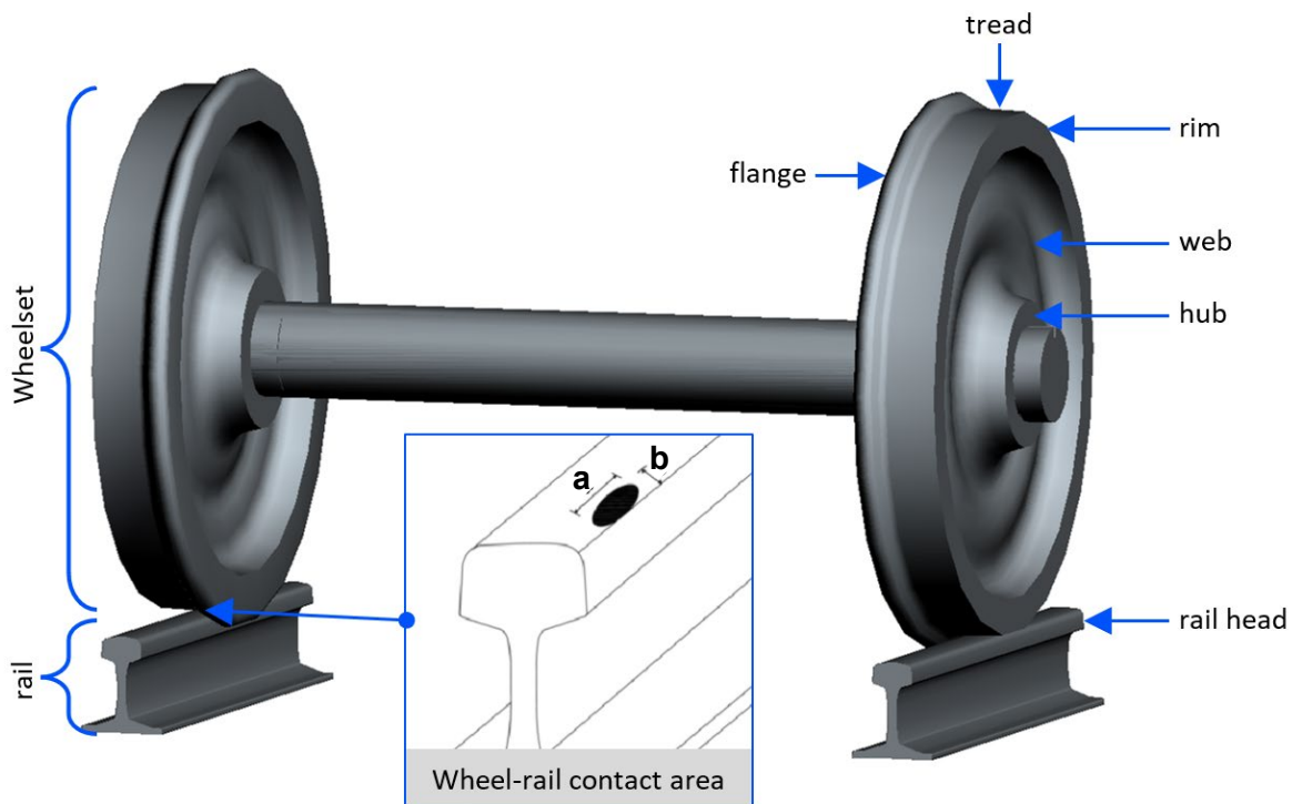
Figure 2: Components of a wheelset with a typical S-type wheel on a UIC 60E1 profile rail, as well as the wheel-rail contact area (from [17] under CC by 4.0)
