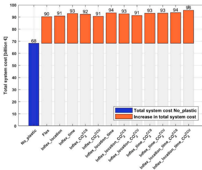
Fig. 4. The total system costs (in billions of Euro) for the investigated scenarios and for the electricity system without electrified production of plastics.
