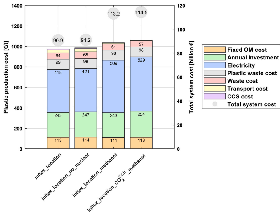
Fig. 10. Breakdown of the modeled plastics production cost into feedstock costs, cost for capture and storage of CO 2 , the annualized investment cost, the fixed O&M costs, electricity cost, and transportation costs (left-hand axis) for the Inflex_location, Inflex_location_NU, Inflex_location_methanol and Inflex_location_CO 2 (CCU)_methanol scenarios. The corresponding total system costs are also shown (right-hand axis).
