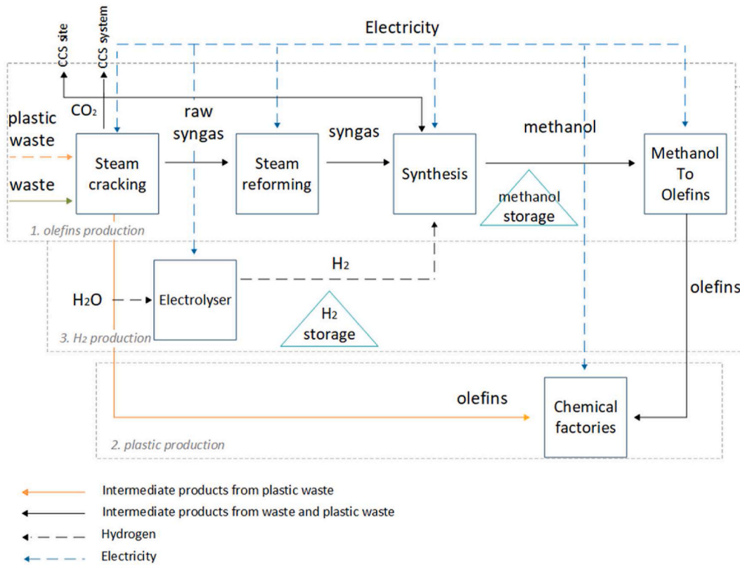
Fig. 1. Schematic of the plastics production process using thermochemical plastic recycling and waste gasification.
