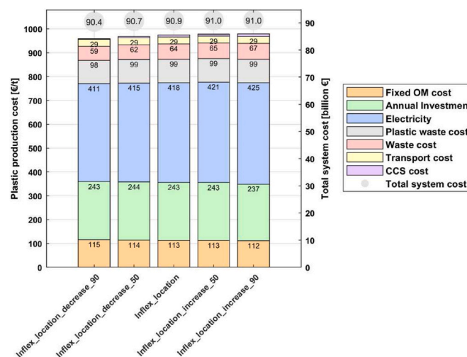
Fig. C1. Breakdown of the modeled plastics production cost into feedstock costs, costs for capture and storage of CO 2 , annualized investment cost, fixed O&M costs, electricity cost, and transportation costs (left-hand axis) for the scenarios with limitations as to location. The corresponding total system costs are also shown (right-hand axis). The cost of hydrogen storage varies between the scenarios, i.e., decreases and increases by 50% and 90%, respectively, as compared to the cost applied in the scenario with limited flexibility as to location: the Inflex_location scenario. The scenarios in which the hydrogen storage cost varies are termed: Inflex_location_decrease_90 , Inflex_location_decrease_50 , Inflex_location_increase_50 and Inflex_location_increase_90 .
