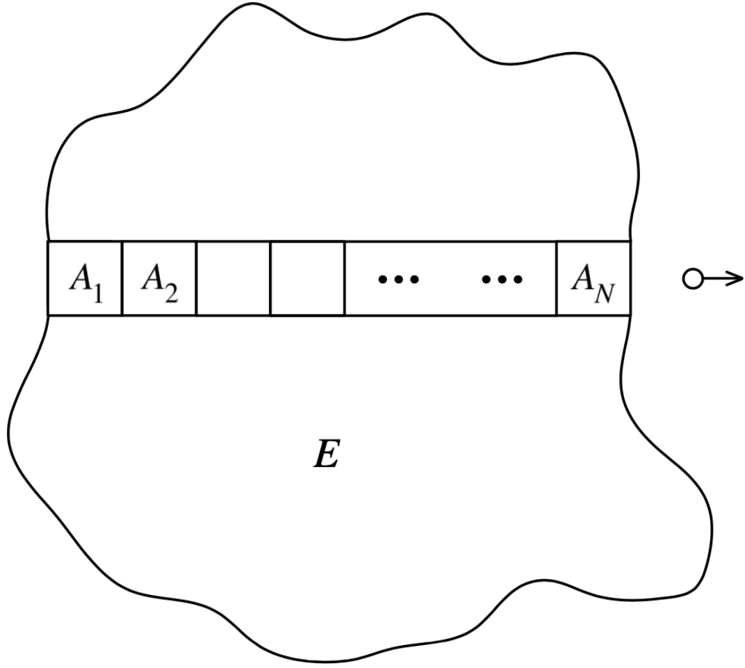
Figure 4. A as a subsystem of the whole measurement apparatus, A \cup E , where E is a large open system with irreversible interaction.
