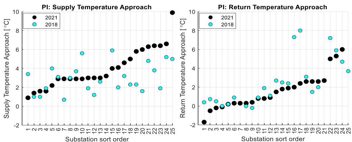
Figure 13: Performance indicators supply temperature approach (left) and return temperature approach (right) for 25 substations from the cooling seasons of 2018 and 2021 (Jangsten, Lindholm, and Dalenbäck 2022a).
