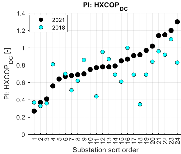
Figure 14: Performance indicator HXCOP DC for 24 substations from the cooling seasons of 2018 and 2021 (Jangsten, Lindholm, and Dalenbäck 2022a).
