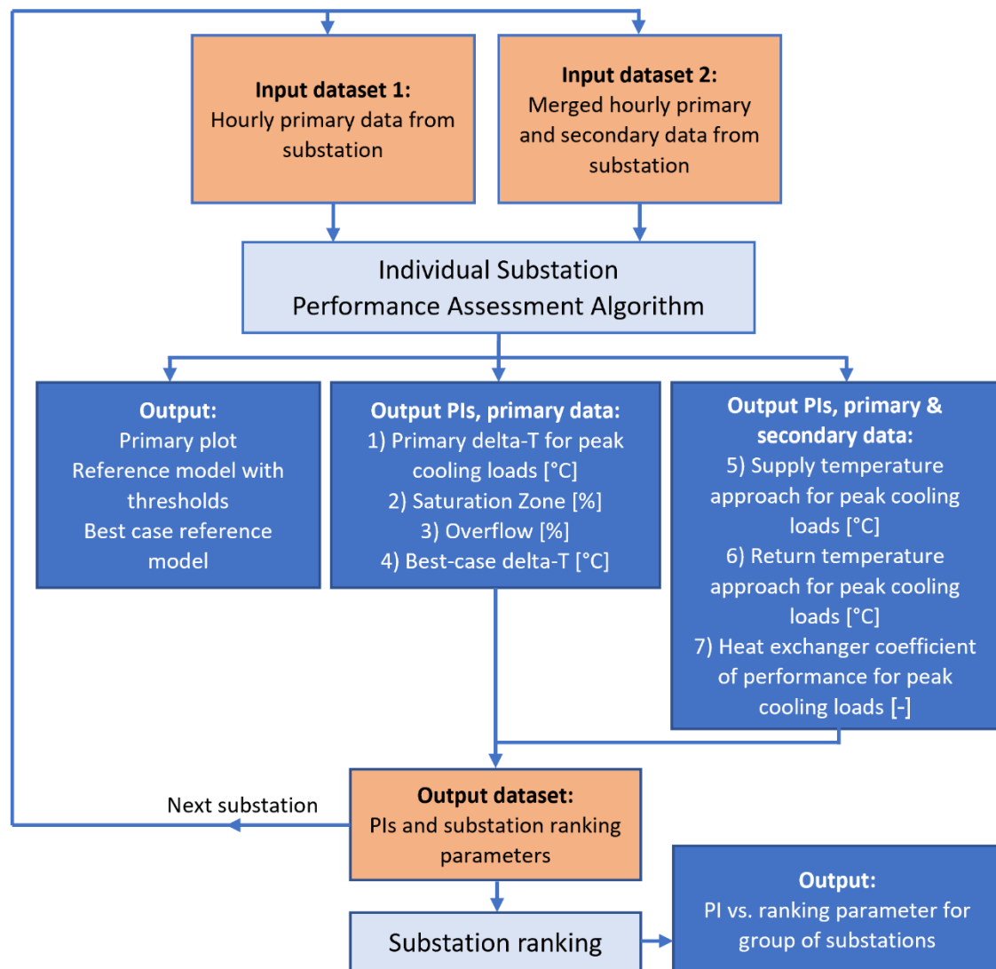
Figure 21: Outline of performance assessment method algorithm with steps and order of calculations along with required inputs and resulting outputs (Jangsten, Lindholm, and Dalenbäck 2022a).
