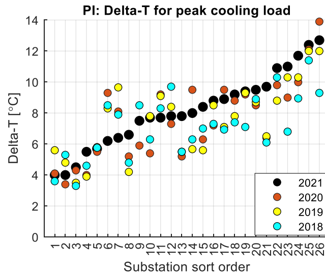
Figure 10: Performance indicator delta-T for peak cooling loads for 26 substations from the cooling seasons of 2018-2021 (Jangsten, Lindholm, and Dalenbäck 2022a).
