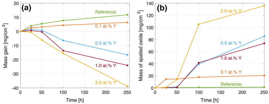
Fig. 2 Mass change plotted against time for Y-doped Mo(Si,Al) 2 materials exposed at 1500 °C, a mass change of sample only, b mass of spalled scale
