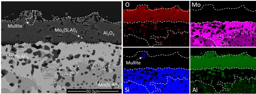
Fig. 3 The reference material after 24 h oxidation. The BSE image shows the \text{Al}_2\text{O}_3 scale with a mullite region, the \text{Mo}_5(\text{Si},\text{Al})_3 layer and the bulk material which is dominated by \text{Mo}(\text{Si},\text{Al})_2 . EDS maps show the distribution of O, Mo, Si (with mullite indicated) and Al. A detached \text{Mo}_5(\text{Si},\text{Al})_3 particle in the \text{Al}_2\text{O}_3 scale is indicated by an arrow
