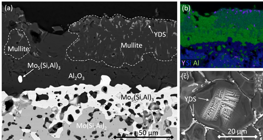
Fig. 6 2 at.% Y after 50 h exposure, a cross-section BSE image with the different phases indicated, b EDS map showing Y, Si and Al, c BSE image of surface \text{Al}_2\text{O}_3 grain with dendritic YDS
