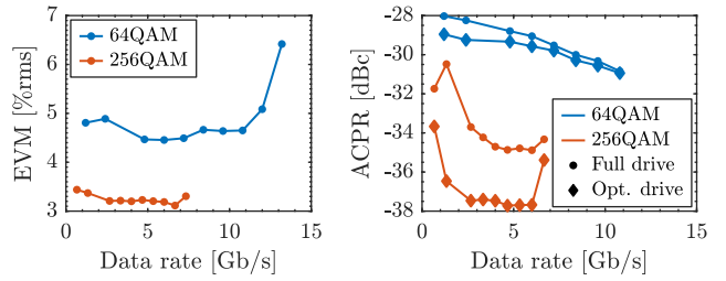
Fig. 6. (a) EVM and (b) ACPR versus data rate for different modulation formats and full/optimum drive slope setting, all with a BER <10^{-3} . Instrument limitations prevent ACPR measurements for the widest-band 64QAM signals.
