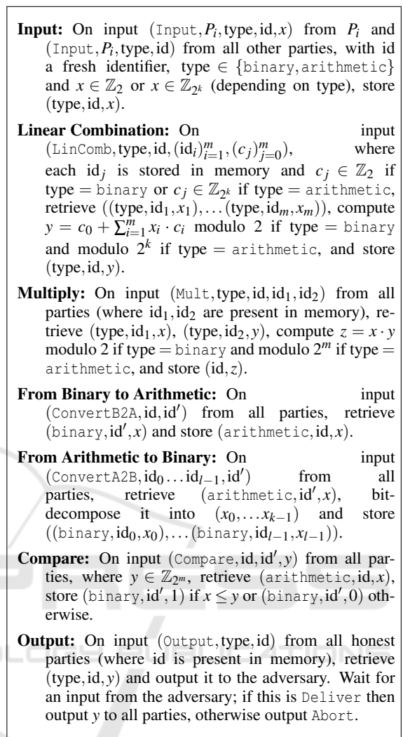
Figure 1: Ideal functionality \mathcal{F}_{AB-MPC} of MPC arithmetic blackbox modulo 2 and modulo 2^k (Escudero et al., 2020).
