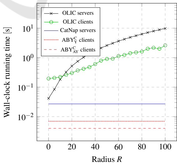
Figure 7: Comparison of CatNap with OLIC, ABY Y C and ABY AY C .
