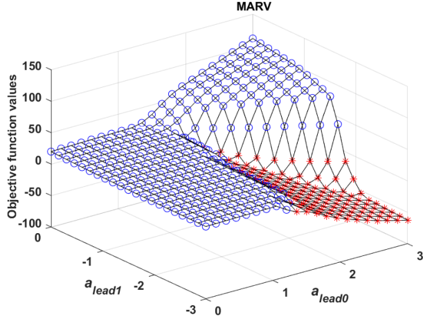
Figure 3.3: Objective function values for combinations of the accelerations (a_{lead0}, a_{lead1}) using MARV semantics, presented in Paper A. Positive values (○) mean that the specification is satisfied, while negative values (*) mean that it is falsified.
