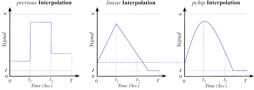
Figure 5.2: Three piecewise input signals with three control points distributed uniformly in time with previous , linear , and pchip interpolation.
