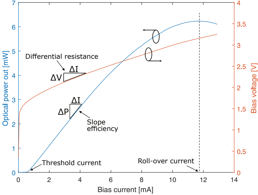
Figure 2.9: IPV plot with some important performance measures marked.
