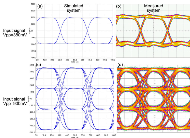
Fig. 4. Input electrical eye diagrams at 28 Gbaud with an ideal 50 \Omega load: (a) simulated, OOK-modulation; (b) measured, OOK-modulation; (c) simulated, PAM4-modulation; and (d) measured, PAM4-modulation.
