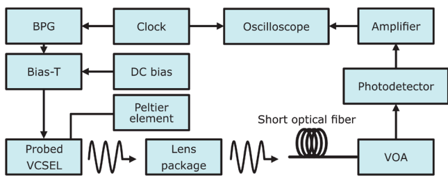
Fig. 3. A block diagram illustrating the experimental setup used in the large-signal performance measurements.
