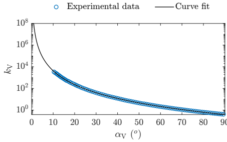
Figure 3.3: Minor loss coefficient of the valve ( k_V ) as a function of valve opening ( \alpha_V ), where 0° is fully closed and 90° is fully open.
