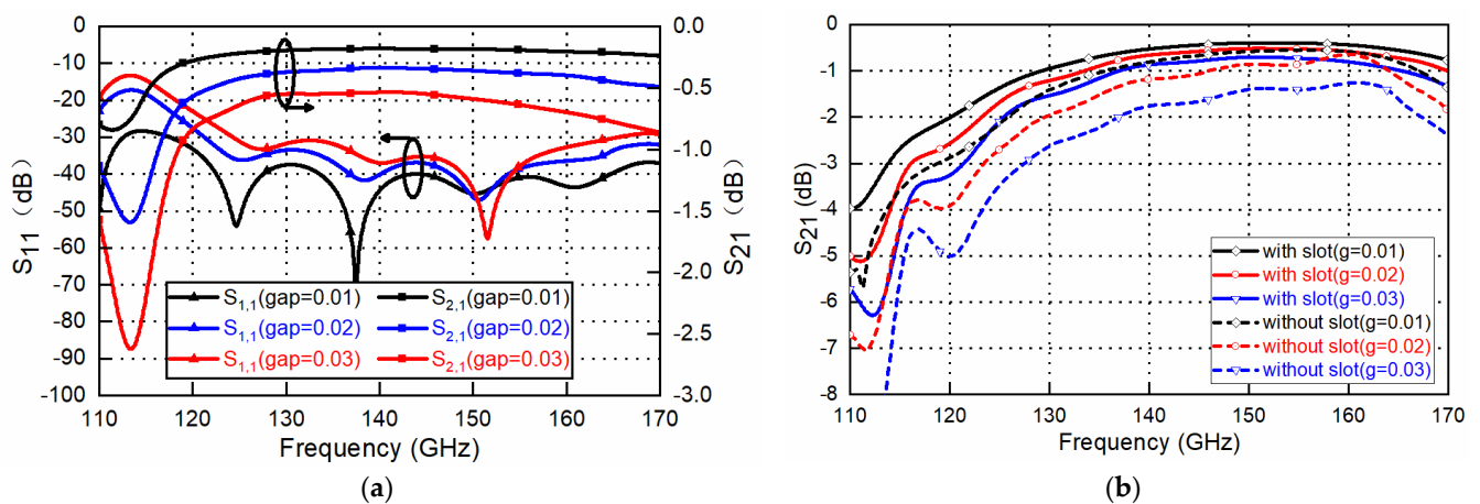
Figure 5. Simulated frequency response of the designed D-band GWG line (a) and with and without rectangular slots along the groove channel (b).
