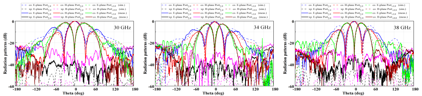
FIGURE 16. Simulated and measured radiation patterns of the proposed feed for Hor-Polar \text{Port}_{\Sigma H} , \text{Port}_{\Delta EH} and \text{Port}_{\Delta HH} .
