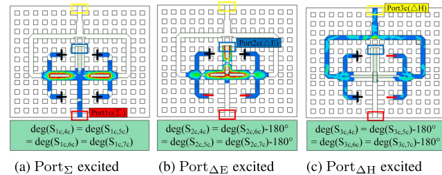
FIGURE 7. Electric field distribution of the proposed monopulse comparator at 34 GHz.
