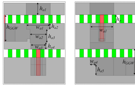
(a) Exploded view (b) Side views from Port 1r (left) and from 2r (right)
