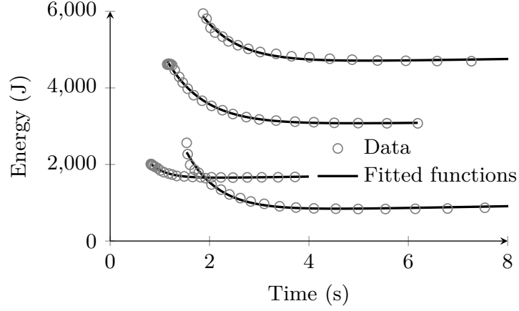
Figure 3.1: Examples of the energy data and fitted functions of four operations.
