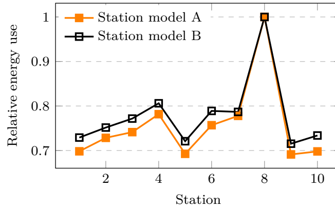
Figure 4.8: The optimized energy for each station for the two station models.
