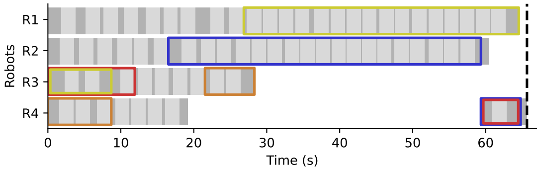
Figure 4.1: A time schedule of the unoptimized welding station, showing the four robots and the execution times of their respective operations. The welding operations are light gray, movement operations are grey, and the deadline is shown as a black dashed line. The colours indicate resource constraints between sequences of operations from different robots. Two sequences of operations with the same colour cannot be executed at the same time.
