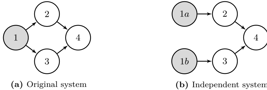
Figure 3.2: An illustration of the independence assumption. The figures represent operations and precedence constraints. Both 1a and 1b have the same distribution of their execution times as 1 but are otherwise independent. The completion times of operation 4 are equal to C_4 = \max(E_1 + E_2, E_1 + E_3) + E_4 and \hat{C}_4 = \max(E_{1a} + E_2, E_{1b} + E_3) + E_4 for the two examples respectively. It can be shown that P(C_4 < t_d) \geq P(\hat{C}_4 < t_d) .
