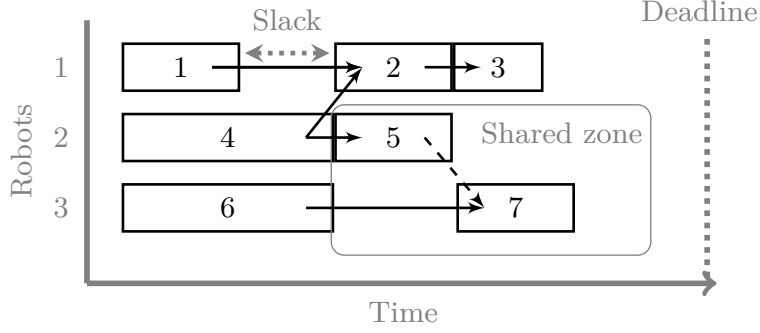
Figure 2.3: An illustrative example schedule of a robot station, containing a set of operations and resources. The operations are shown as numbered boxes and the solid arrows between them are necessary precedence constraints. The station contains four resources: three robots and one shared zone. The robots are listed to the left. The operations on the same row as a robot require that robot to execute. Operation 5 and 7 also require the shared zone to execute. Only two operation orders are possible: the one where Operation 5 precedes Operation 7 (which is shown) or the other way around. The additional precedence constraint determined by the control strategy and related to the shared zone is shown with a dashed arrow.
