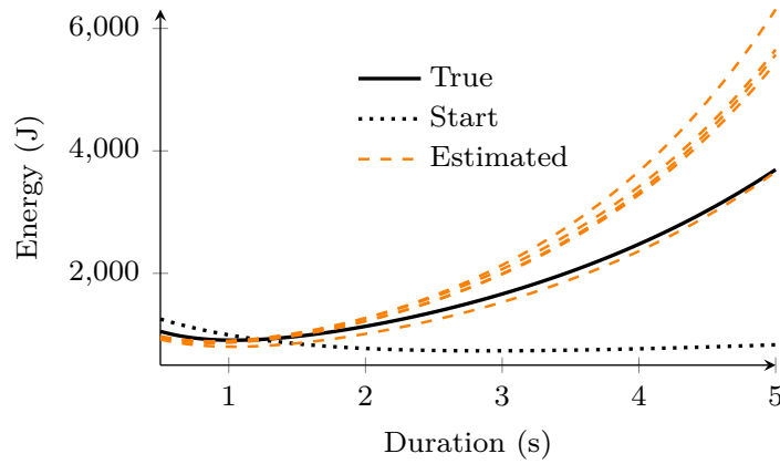
Figure 5.4: The energy function of the move operation with the start, estimated and true parameters values.
