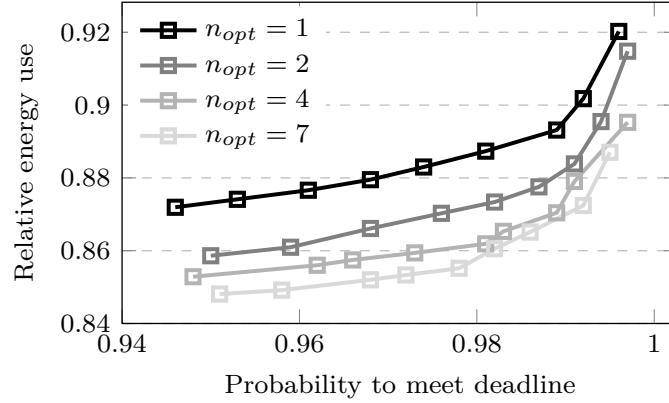
Figure 5.2: The relative energy use as a function of the simulated probability to meet the deadline, for some values of n_{opt} .
