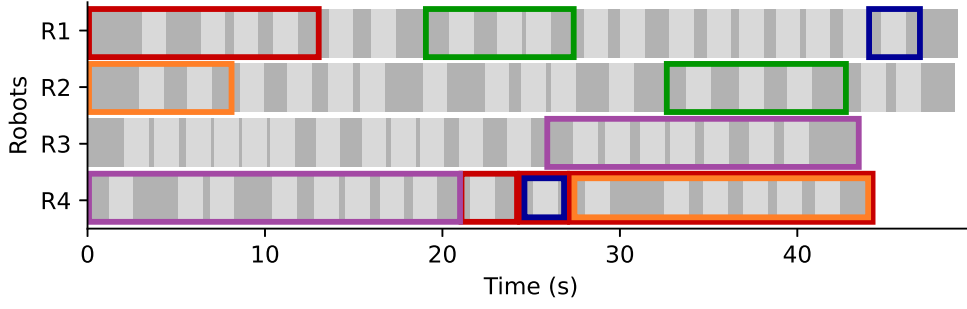
Figure 4.5: A time schedule of a robot station of the same type as shown in Fig. 4.1. The execution times of the operations shown in the schedule are the mean values for the welding operations and the lower bounds \underline{d}_i for the movement operations.
