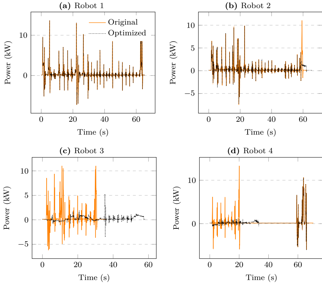
Figure 4.3: The power use of the original and optimized settings for the four robots.
