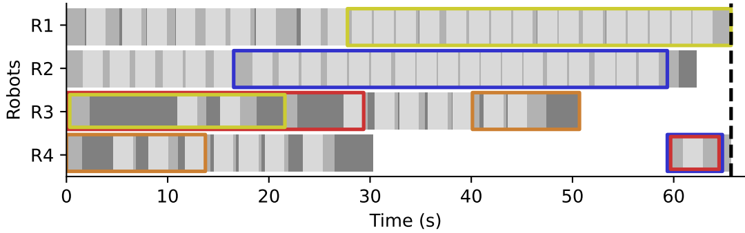
Figure 4.2: A time schedule of the optimized welding station. The darkest gray areas show the execution time extensions (compared to \underline{d}_i ) after the optimization. Otherwise, the notations are the same as in Fig. 4.1.
