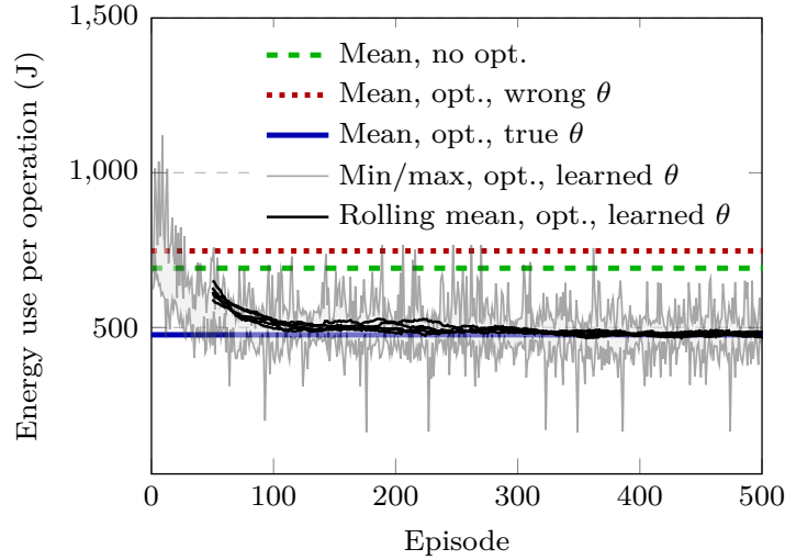
Figure 5.3: The average energy use per operation and episode of the experiment.
