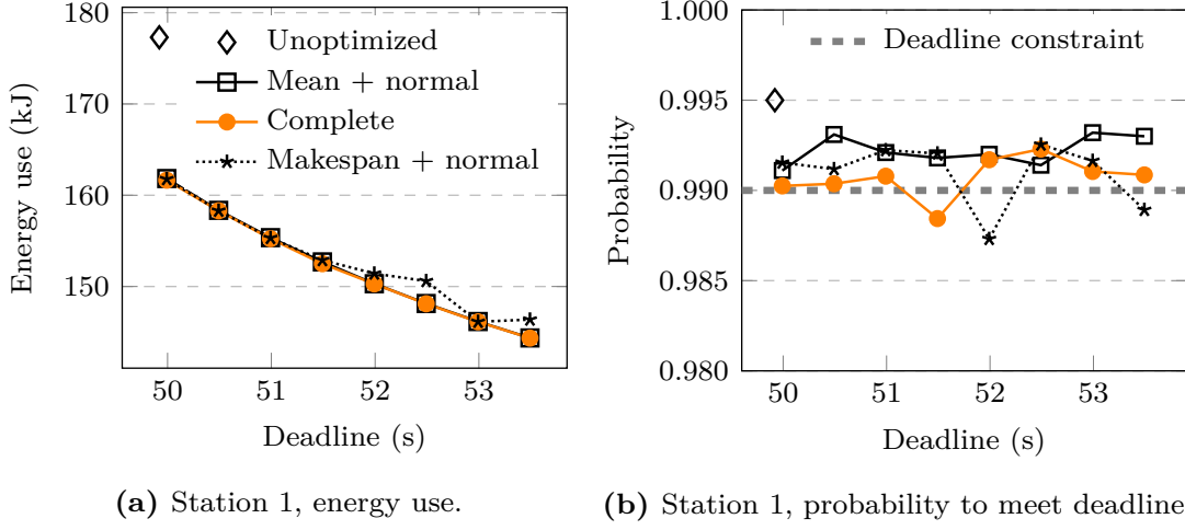
Figure 4.6: The simulated energy use and probability to meet deadline for one of the three stations before and after optimization.
