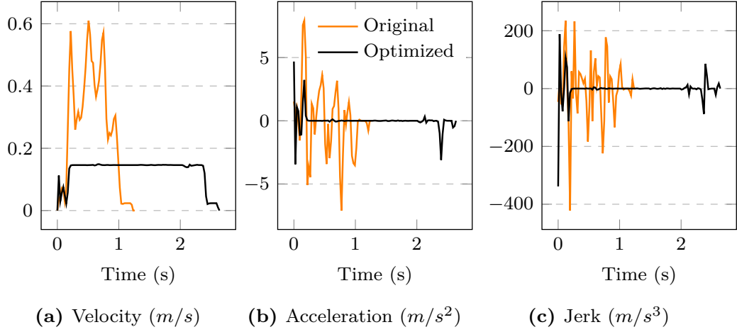
Figure 4.4: The velocity, acceleration, and jerk of one operation with the original and optimized settings
