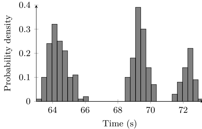
Figure 2.2: The distribution of the execution time of a welding robot in an automotive factory.
