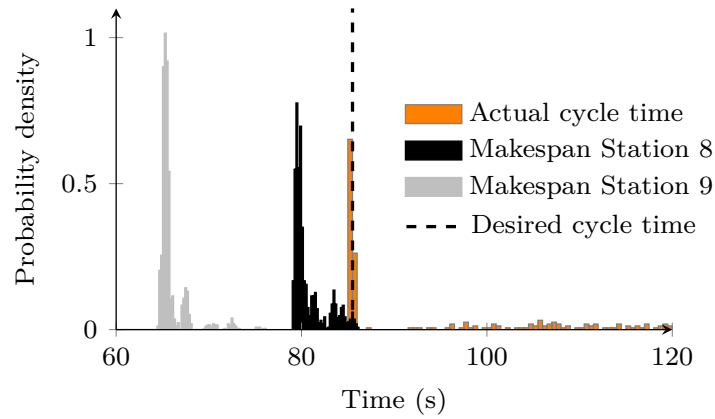
Figure 2.5: The distributions of the makespans of two stations together with the actual and desired deadline for a production line in an automotive factory.
