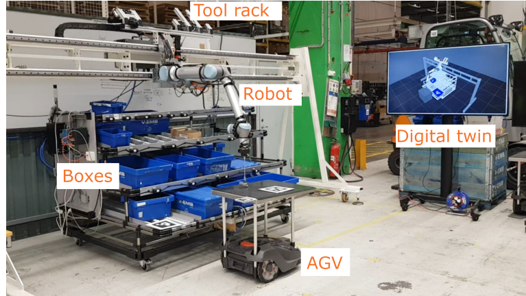
Figure 5.1: The kitting station used as a case study.
