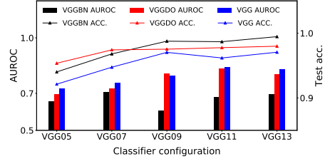
Fig. 8: Effect of regularization on AUROC
