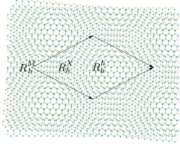
Figure 4.1: Schematic of a twisted bilayer TMD superlattice.
