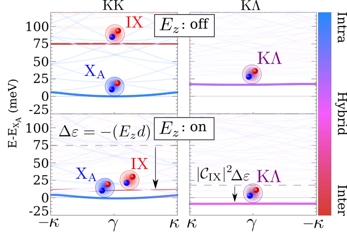
Figure 4.3: Exciton band structure for R-type stacked MoSe 2 homobilayer for the bright KK (left) and dark KA excitons (right). Multiple moiré subbands are shown in faded colors. Only the interlayer and the hybrid exciton exhibiting a dipole moment become red-shifted in presence of an electrical field (lower panel). Dashed lines indicate the original position of the corresponding excitons without an electrical field. The calculation is performed for a twist angle of \theta = 2^\circ and an electrical field of E_z = 0.1 V/nm.
