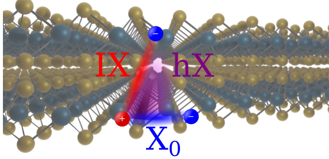
Figure 1.2: Illustration of bilayer TMD with a hybrid exciton hX made out of an interlayer component IX and an intralayer component X_0 .
