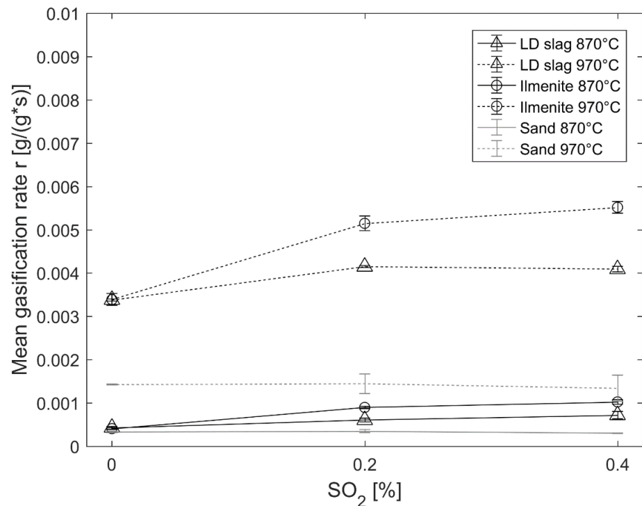
Figure 7. Mean gasification rate “r” between 0.3 < X_c < 0.7 for LD slag, ilmenite, and sand at different temperatures and concentrations of SO_2 .
