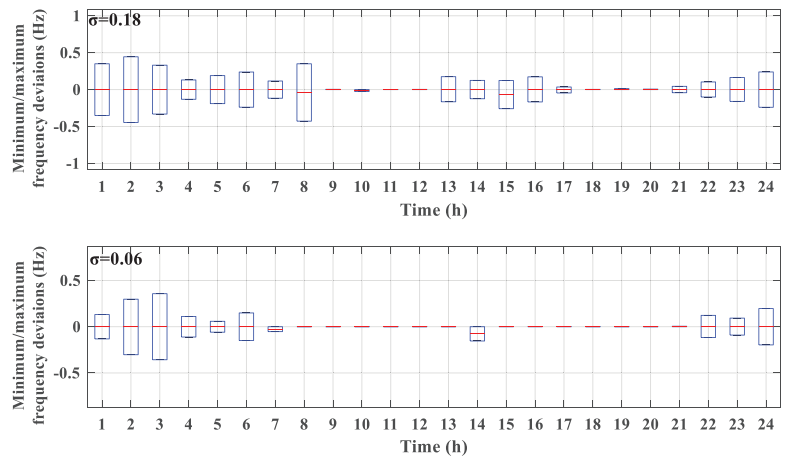
FIGURE 15 Frequency nadir (negative values) and frequency zenith (positive values) for uncertainty budgets of 0.18 and 0.06
