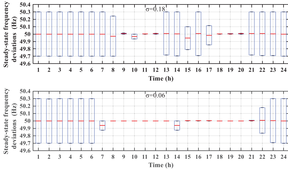
FIGURE 13 Steady-state frequency deviations for uncertainty budgets of 0.18 and 0.06
