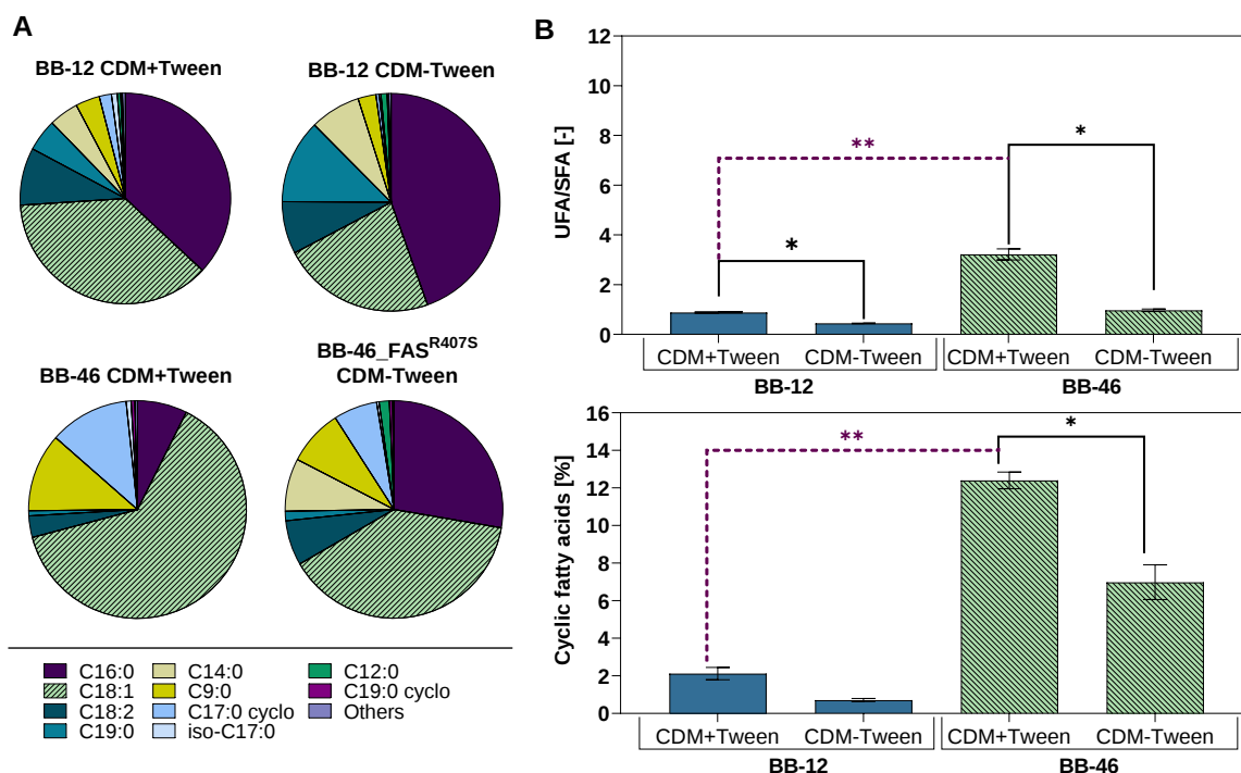
Figure 13: Fatty acid profile of BB-12 and BB-46 in CDM containing Tween® 80 (CDM+Tween), as well as of BB-12 and BB-46_FAS R407S in CDM without Tween® 80 (CDM-Tween). The fatty acid profile was analyzed in stationary phase. A. Content of individual fatty acids in the cell membrane. Each value represents the mean of a triplicate. B. Fatty acid profile characterization. Each value represents the mean of a triplicate \pm standard deviation. UFA/SFA: ratio of unsaturated to saturated fatty acids. The UFA/SFA ratio was calculated without considering cyclic fatty acids. Significant differences between means were tested by a multiple unpaired t -test with CDM-Ref serving as reference; * p adj < 0.05, ** p adj < 0.005 (adapted from Figure 5 in Paper IV ).
