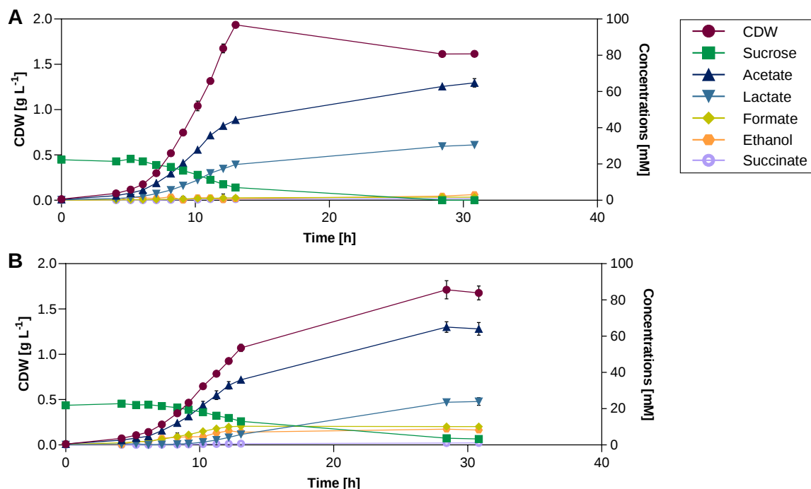
Figure 9: Growth dynamics and metabolite profiles of BB-12 (A) and BB-46 (B). Cultivations were conducted in crimp-top serum bottles under anaerobic conditions (80% \text{N}_2 and 20% \text{CO}_2 ) at 37^\circ\text{C} in CDM supplemented with 10 \text{ g L}^{-1} sucrose and a starting pH of 6.5. Each data point represents the mean of biological triplicates \pm standard deviation.
