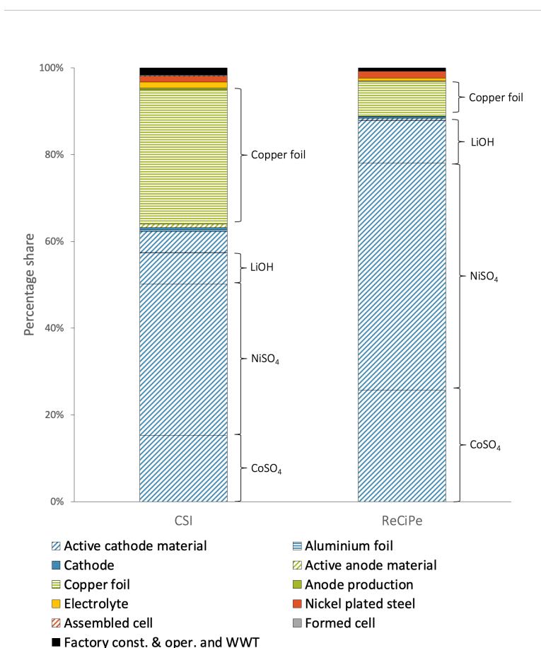
Figure 7: Resource use impacts of large-scale LIB production assessed using two different mineral resource scarcity assessment methods
