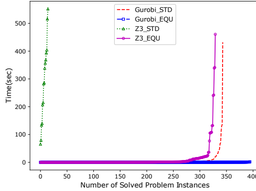
Figure 3.9: Comparison of different model formulations using Z3 and Gurobi over a benchmark set of the BCP.
