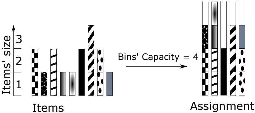
Figure 2.2: Illustration of a possible assignment for a bin sorting problem.
