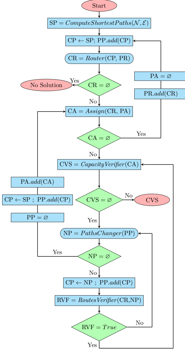
Figure 2: Flowchart of ComSat algorithm.
