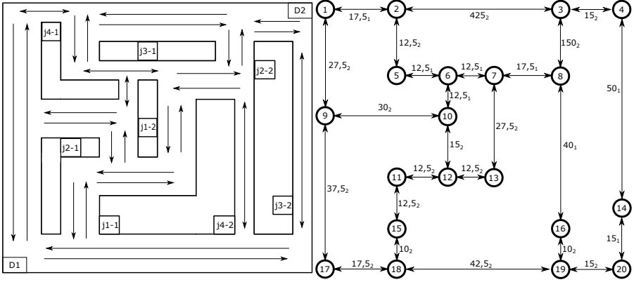
Figure 4.1: A hypothetical plant layout taken from paper D and its abstraction into a graph.
