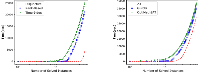
Figure 3.8: Comparison of different model formulations (left) and different solvers (right) over a benchmark set of the JSP.
