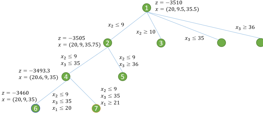
Figure 3.3: Illustration of branch and bound steps.
