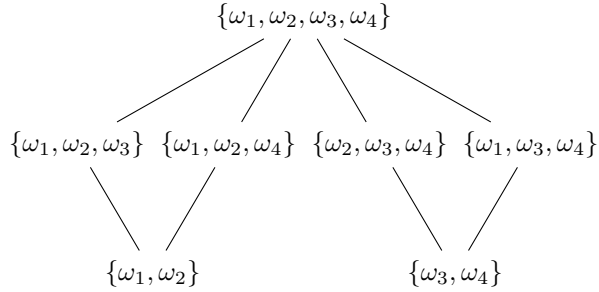
Figure 3.7: Lattice of the Unsat Core set of Scenario 3.
