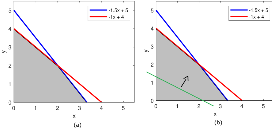
Figure 3.1: Illustration of the feasible region (a) and objective function (b) for the LP example.
