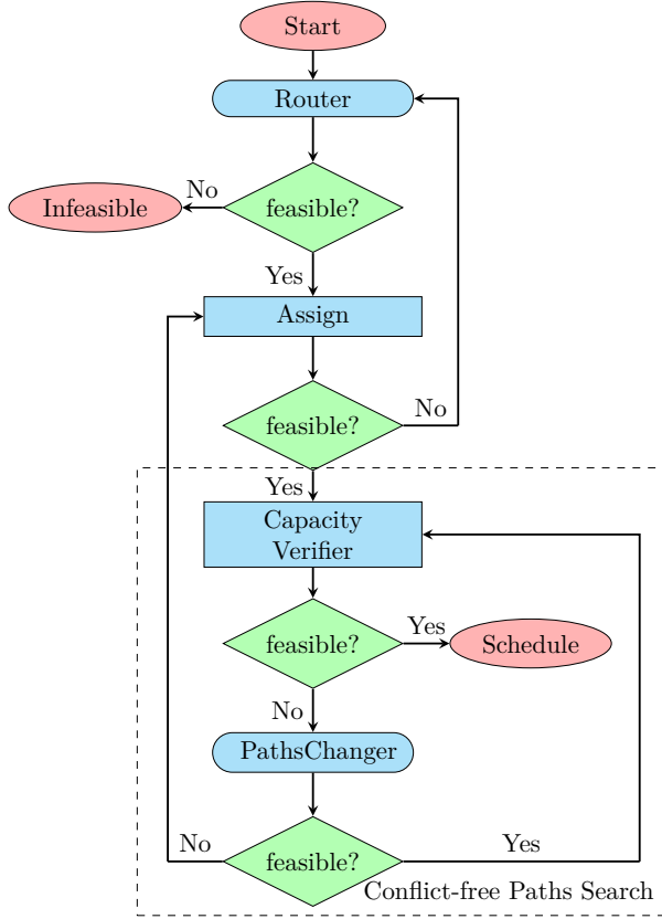
Figure 1: Flowchart of ComSat.
