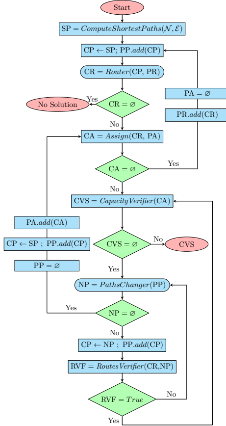
Figure 5.6: Flowchart of ComSat. The Router and PathsChanger algorithms are put in rounded corner boxes, to remark that they are optimization problems.
