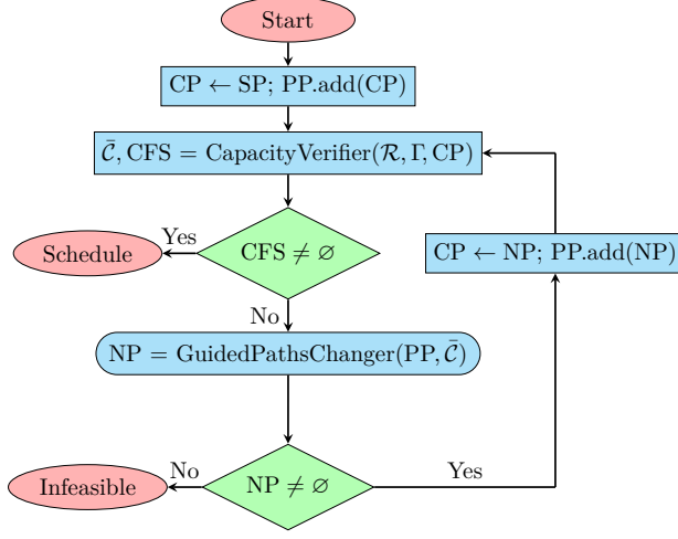
Figure 2: Flowchart of the MUC-Guided-CFPS .
