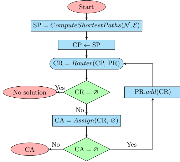
Figure 3: Flowchart of C-ComSat.
