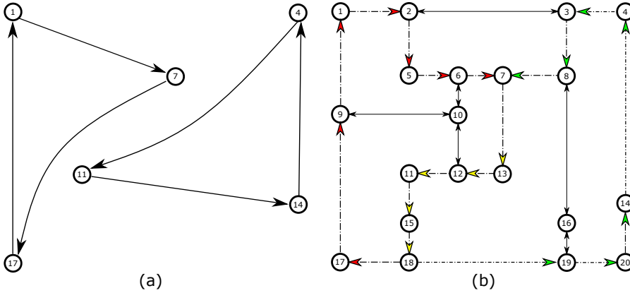
Figure 5.4: Routes (a) are verified against capacity constraints on the actual plant layout (b).
