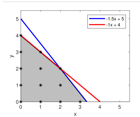
Figure 3.2: Illustration of the feasible region when the integrality constraint applies.
