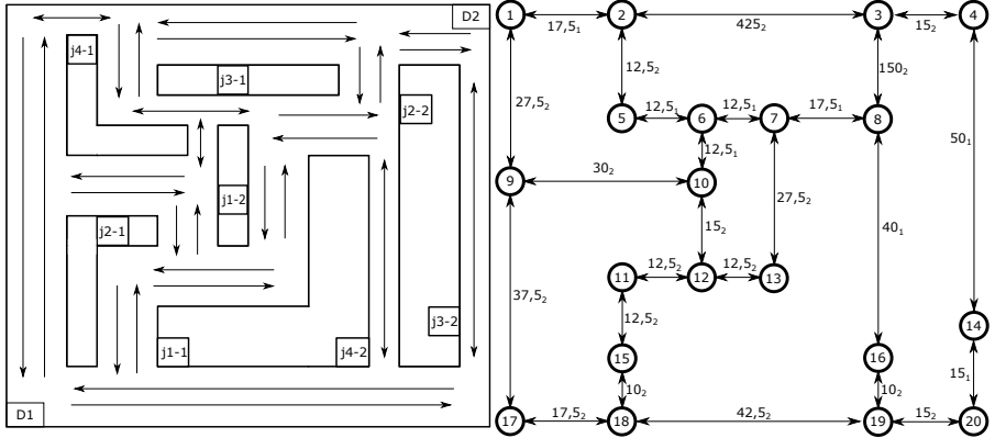
Figure 1: Problem instance of the CF-EVRP picturing a hypothetical plant (left) where two depots ( D1 , D2 ) accommodate four vehicles ( v1 , v2 , and v3 , v4 respectively), available to execute four jobs ( j1 , j2 , j3 , j4 ), each composed by two tasks (1, 2). The plant road segments are abstracted into a strongly connected, directed, weighed graph (right).
