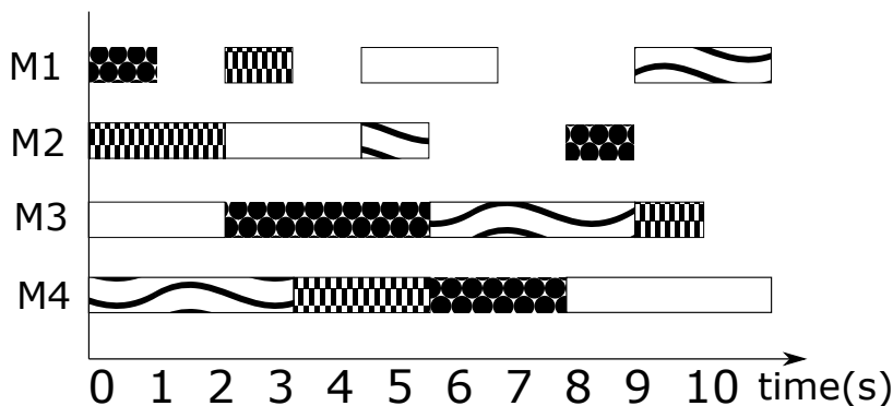
Figure 2.1: Illustration of a possible solution to a job shop problem.
