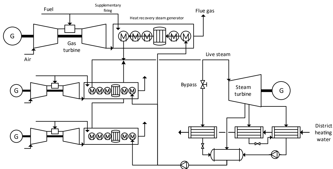
Figure 3.5. Process diagram depicting the combined cycle reference plant. Source: Adapted from Paper III.
