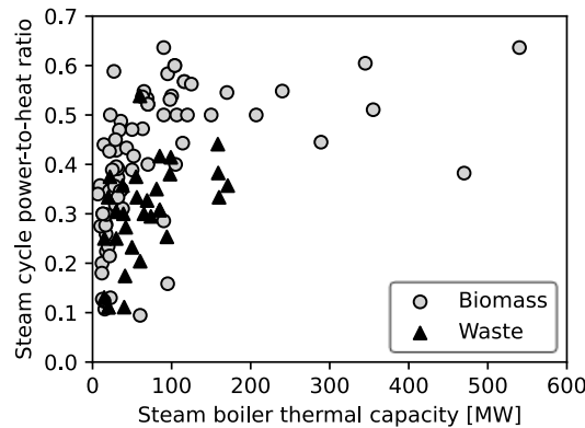
Figure 3.2. Characterization of the 110 Swedish CHP plants that combust waste or forest residues, with respect to boiler thermal capacity, steam cycle power-to-heat ratio and fuel type. Each marker represents one plant. Source: Paper I.
