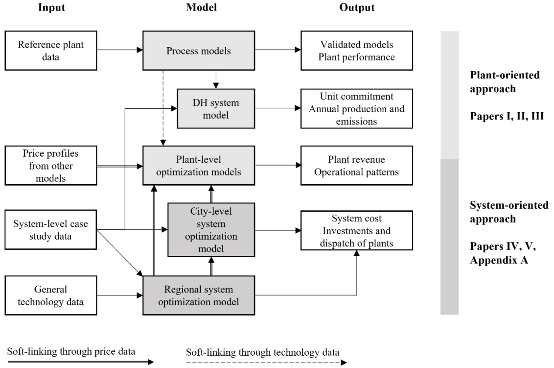
Figure 2.2 Modeling framework overview. DH, district heating.
