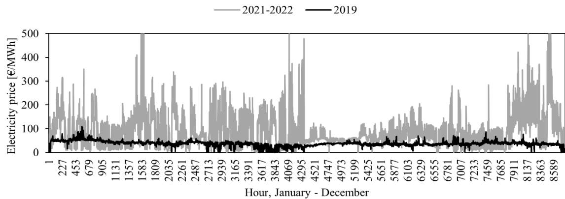
Figure A.1. Import electricity price profiles, based on price data for the SE3 area, for year 2019 and the period July 2021 – June 2022.
