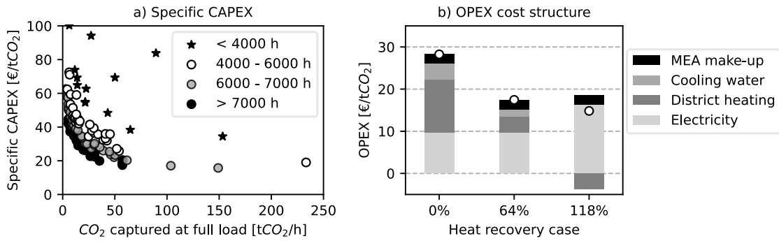
Figure 6.4. a) Specific capital cost (CAPEX) of the CO 2 capture and conditioning plant for CHP plants as a function of plant size (CO 2 flow treated) and full load hours. Each point represents one CHP plant. Note that the y-axis is cut at 100 €/tCO 2 . b) The cost of operating a CHP plant with carbon capture (OPEX) under three heat recovery scenarios (Section 3.4). The white dots indicate the net OPEX. Source: Adapted from Paper I.
