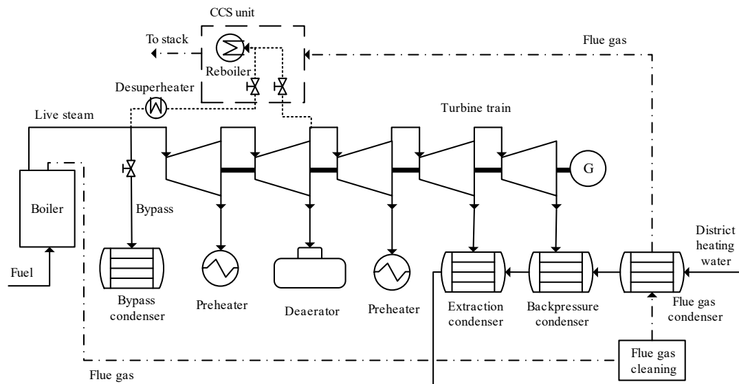
Figure 3.4. Process schematic of a CHP steam cycle. The feed water system is omitted for clarity. Dotted lines represent steam extraction alternatives that can be retrofitted to drive a carbon capture reboiler. Source: Adapted from Paper I.
