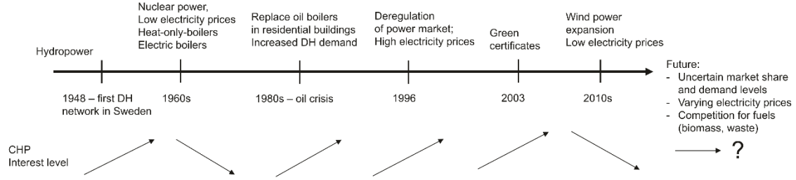
Figure 3.1. Timeline of major energy system developments in Sweden (1950-2020) that have influenced the incentives for CHP plants. DH, district heating.
