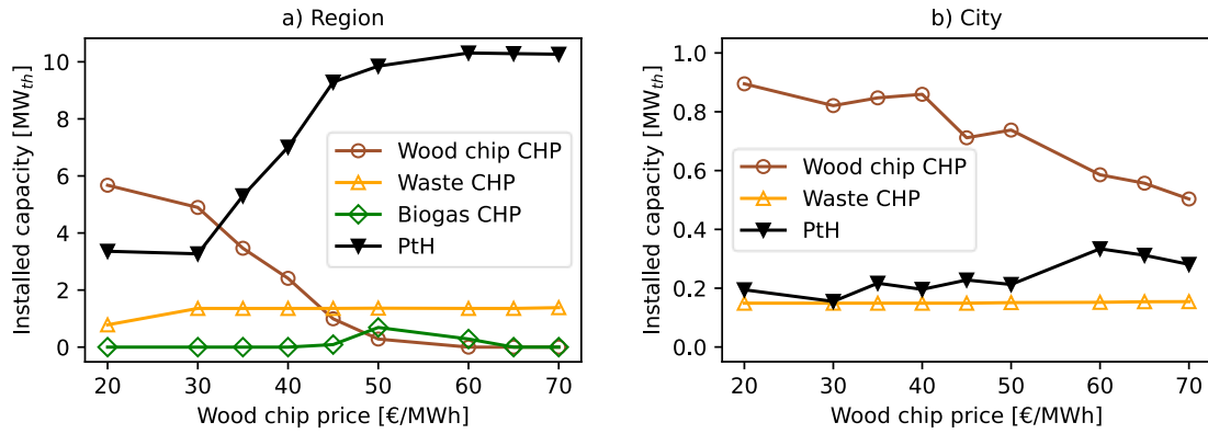
Figure 6.1. Optimal investments in CHP capacity and power-to-heat technologies as a function of wood chip price, in a) the SE3 region and, b) the City of Gothenburg. Source: a) Paper IV, b) based on Paper V with complementary model runs. Please note the different scales on the y-axes.
