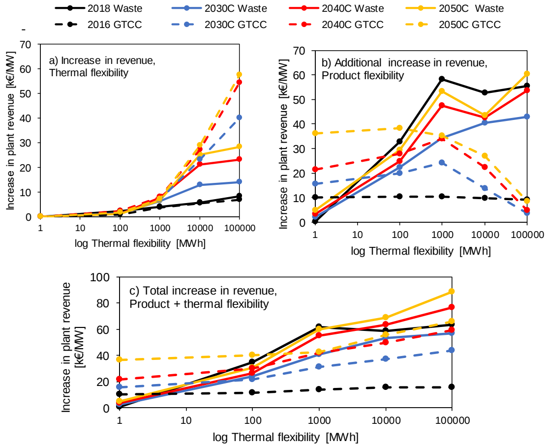
Figure 6.3. a) The annual plant revenue increase per installed electric capacity as a function of thermal flexibility (TES storage capacity), for different electricity price scenarios. b) The additional increase in plant revenue when product flexibility is added to thermal flexibility. c) The total increase in revenue from product and thermal flexibility is given by the sum of a) and b). Solid lines represent the waste-fired plant, and dashed lines the combined cycle (GTCC). Note the logarithmic scale on the x-axes. Source: Paper II and Paper III.
