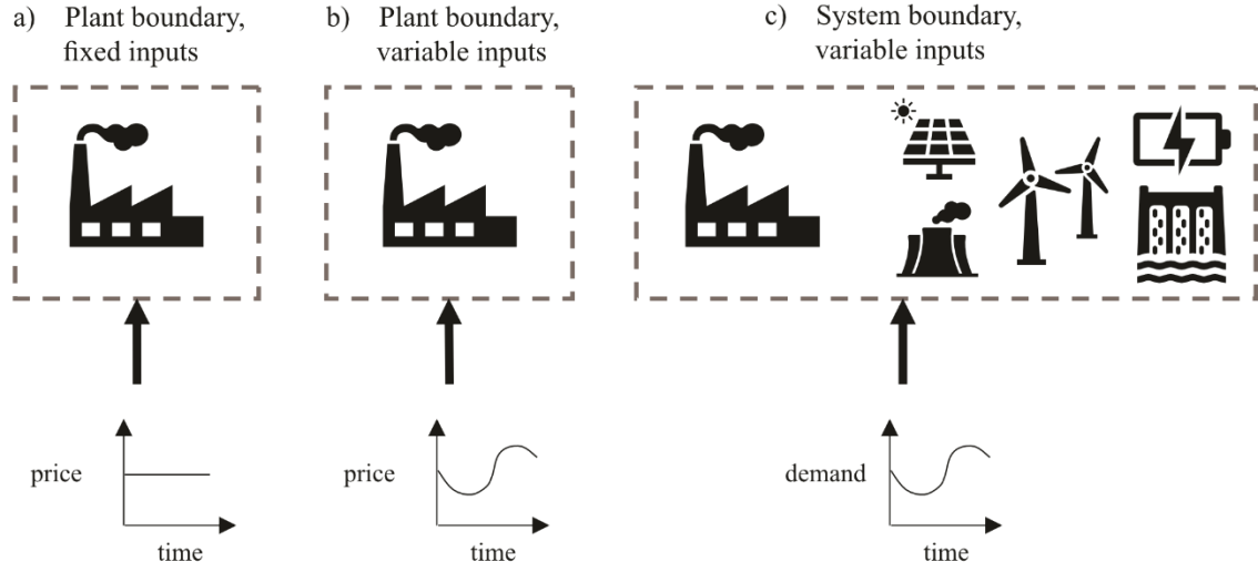
Figure 2.1. System boundaries that can be applied in techno-economic assessments. a-b) Plant-level boundaries with fixed (a) or variable (b) input data. c) System-level boundary with variable input data, that takes into account interaction between technologies.
