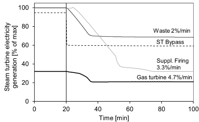
Figure 4.2. Steam turbine electricity generation responses when the thermal input to the steam cycle decreases from full to minimum load, for a waste-fired steam cycle, gas turbine and supplementary firing load changes. The dashed line represents the response from steam flow regulation through a turbine bypass in the waste-fired steam cycle. The ramp rates are indicated by the labels, in load-%/min of nominal capacity. The ramp is initiated at time = 20 minutes, indicated by the vertical line. Source: Paper III and Refs [129,130].
