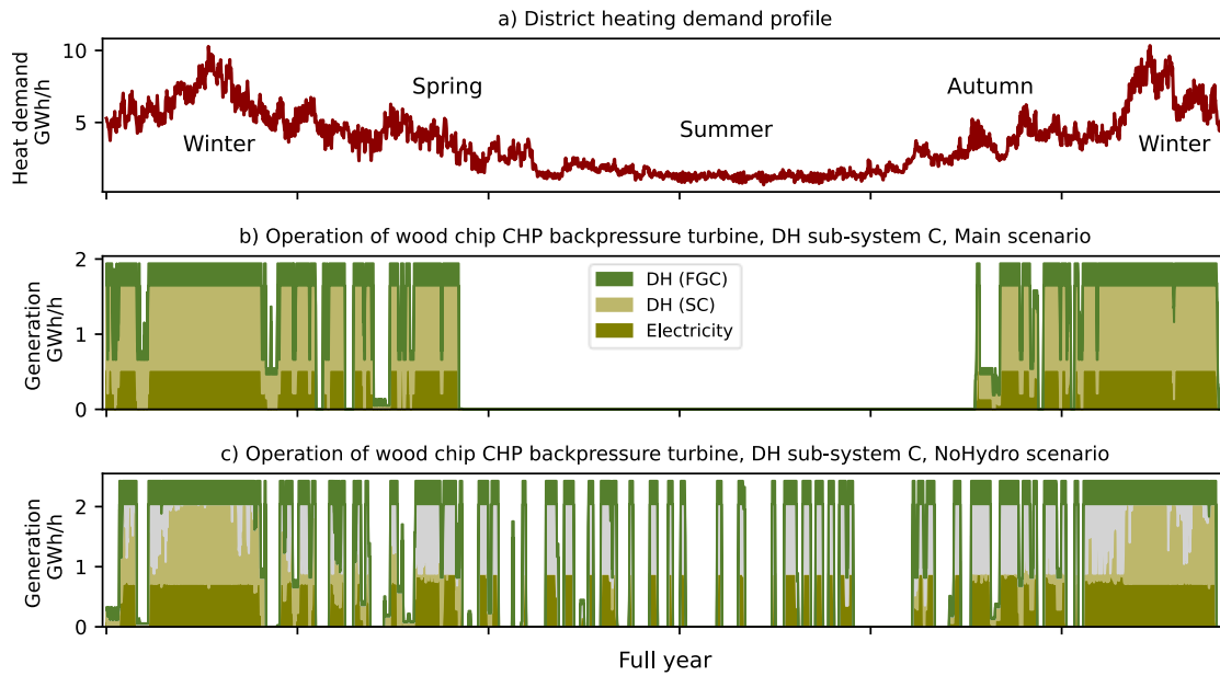
Figure 5.4. a) District heating demand profile for one year. b-c) Optimal dispatch of biomass (wood chip) CHP plants in the (b) main scenario (current biomass price level and access to hydropower), (c) scenario without hydropower. The grey color in panel c represents cooled heat (condensing operation). DH, district heating; FGC, flue gas condenser; SC, steam cycle. Source: Based on the modeling in Paper IV.
