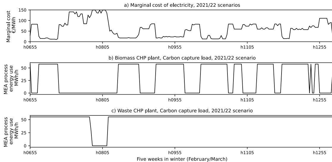
Figure 5.3. a) Marginal cost of electricity in the modeled 2021/22 scenario. b-c) MEA process energy consumption when retrofitted to the b) biomass CHP plant, and c) waste-fired CHP plant. The figure shows five weeks in winter (February/March). Based on the modeling in Appendix A.
