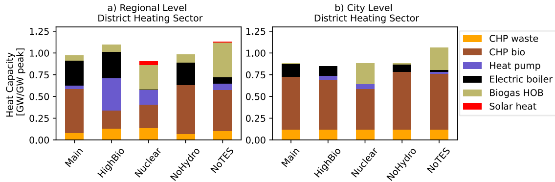
Figure 6.2. Optimal normalized investments in heat generation capacity in a) the SE3 region and, b) the city of Gothenburg. Cases: Main: current biomass price. HighBio: biomass price doubled. Nuclear: current capacity of nuclear power is forced into the regional system. NoHydro: no hydropower available. NoTES: to thermal energy storage available. Source: Based on Paper IV and V, with complementary model runs.
