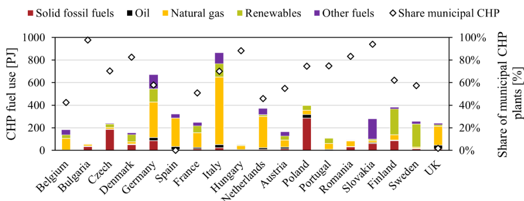
Figure 3.3. CHP plant fuel use in 2015 in EU countries (countries with <50 PJ fuel use are excluded). The fuel use is for both municipal and industrial CHP plants, but the secondary axis indicates the share of municipal plants. “Other fuels” include amongst others industrial wastes and coal gases. Based on Ref [102].
