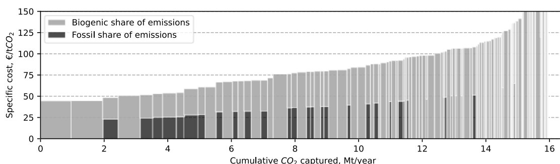
Figure 6.5. Marginal cost of carbon capture from Swedish CHP plants, including cost of capture, liquefaction and compression, and truck transport to an intermediate storage hub. Each bar represents one CHP plant, distinguishing between biogenic (gray) and fossil (black) emissions. Source: Adapted from Paper I.
