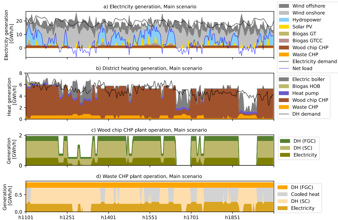
Figure 5.1. Optimal dispatch of the: a) electricity sector, b) district heating sector, c) biomass (wood chip) CHP plant, and d) waste-fired CHP plant, during five weeks in springtime. DH, district heating; FGC, flue gas condenser; SC, steam cycle turbine condenser. Source: Based on Paper IV.
