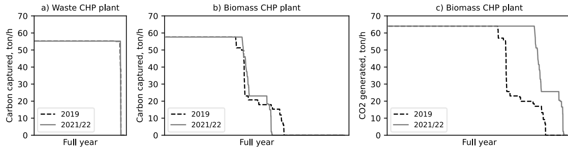
Figure 5.2. Carbon capture plant load duration curves for the capture processes when applied to a) a waste-fired CHP plant, and b) a biomass CHP plant. Panel c) shows the duration curve of CO 2 generated by the biomass CHP plant. The data are arranged from highest to lowest load, i.e., not in chronological order. Based on the modeling in Appendix A, where the 2019 and 2021/22 scenarios are explained.
