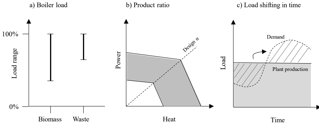
Figure 4.1. Dimensions of CHP plant flexibility. a) One-dimensional flexibility in the form of boiler load range. b) Two-dimensional flexibility obtained from the ability to vary product ratios ( \alpha ) in addition to boiler load variation. c) Flexibility in time (load shifting) enabled by energy storage.
