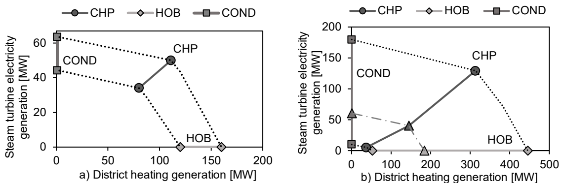
Figure 4.3. Steam cycle load range expansion from product flexibility, for the a) waste-fired, and b) combined cycle reference plants. CHP, combined heat and power generation; HOB, heat-only generation; COND, electricity-only generation. Dotted lines mark the feasible operating regions. Triangles mark combined cycle performance at nominal gas turbine load without supplementary firing. Note the different scales on the axes. Source: Adapted from Paper II and Paper III.
