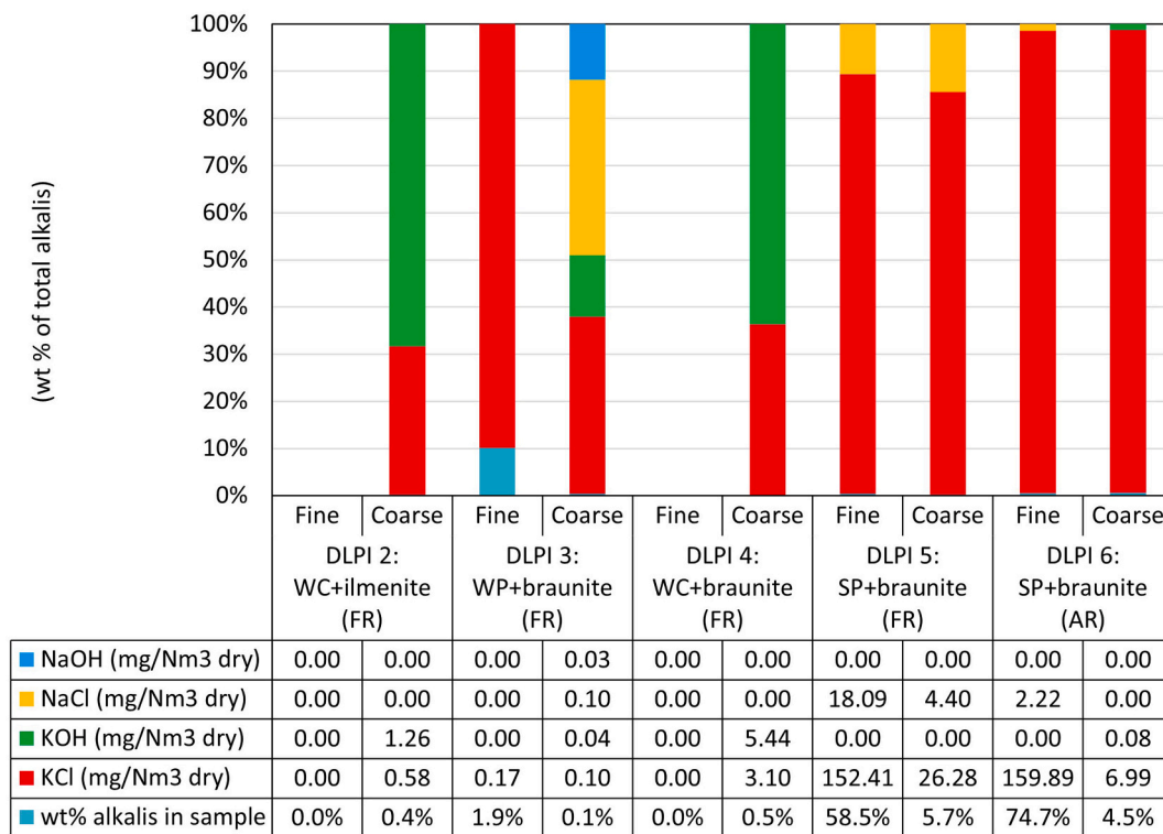
Fig. 17. Impactor sample alkali speciation.
