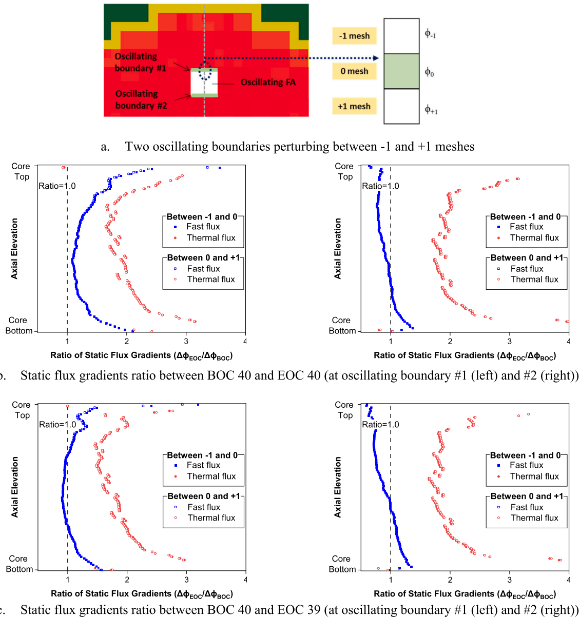
Fig. 23. Comparison of ratios of static flux gradients.
