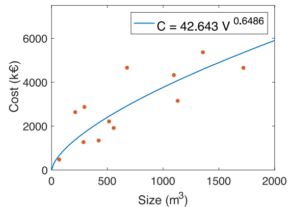
Fig. 7. Cost function for columns, including internals, material: welded SS316. The red dots represent column costs estimated in previous work (Biermann et al., 2019; Gardarsdóttir et al., 2019; van der Spek et al., 2017). The blue line shows the power function fitted to the data points. The sizing parameter ( V ) for columns is the volume in \text{m}^3 .
