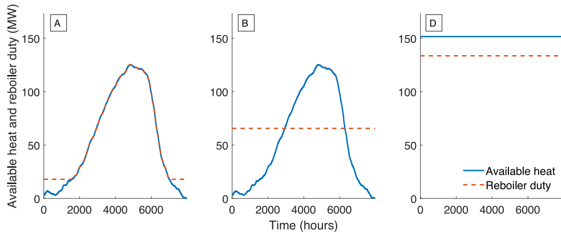
Fig. 5. Available heat and reboiler duty for configurations A, B and D respectively in the case study. Heat load curves were based on the work by Martinez Castilla et al. (2019) .
