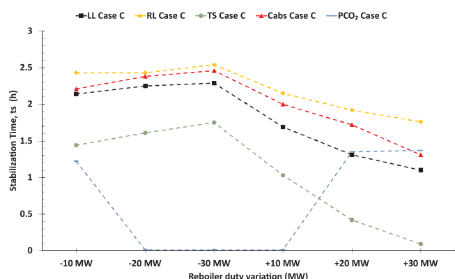
Fig. 11. Stabilization times (hour) of the main process variables for different steps in reboiler heat load for Case C. LL, Lean Loading; RL, Rich Loading; TS, temperature in the stripper bottom; C_{abs} , CO 2 capture rate in the absorber; and P_{CO_2} , CO 2 produced in the stripper.
