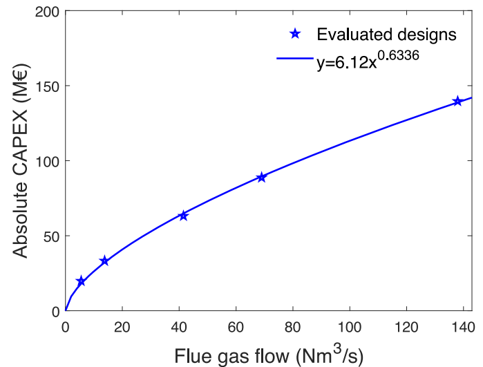
Fig. 6. CAPEX (M€) as a function of flue gas flow ( \text{Nm}^3/\text{s} ). The CAPEX was evaluated for five designs (indicated by the star symbols), to which a power function was fitted to set up the cost function.
