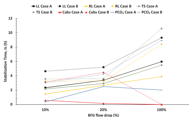
Fig. 9. Stabilization times (hours) for step-changes in the blast furnace gas flow. Solid lines represent Case A (summer) and dashed lines represent Case B (winter). LL, Lean Loading; RL, Rich Loading; TS, temperature in the stripper bottom; C_{abs} , CO 2 capture rate in the absorber; and P_{CO_2} , CO 2 produced in the stripper.
