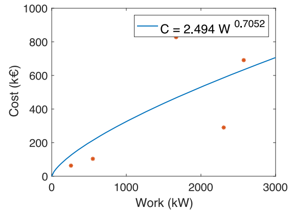
Fig. 16. Flue gas fan cost function, material: carbon steel. The sizing parameter (W) for the flue gas fan is the required work (kW).
