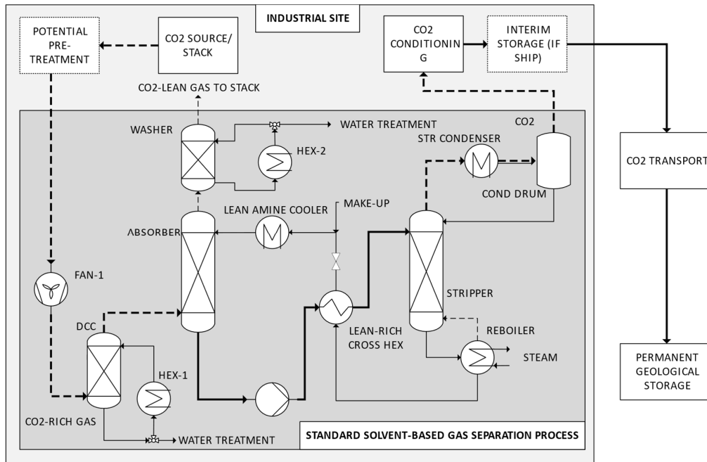
Figure 3-2: Process flow diagram of the standard gas separation solvent process placed in the context of the industrial site and the full CCS chain, i.e., including the off-site CO 2 transport and permanent geologic storage.
