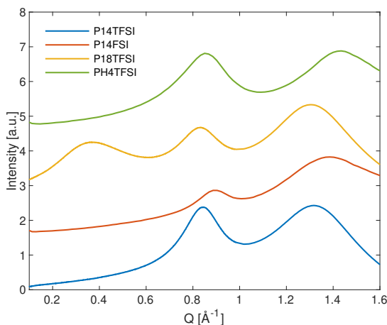
Figure 6.2: SAXS patterns for ionic liquids in the pyrrolidinium family investigated in this thesis.
