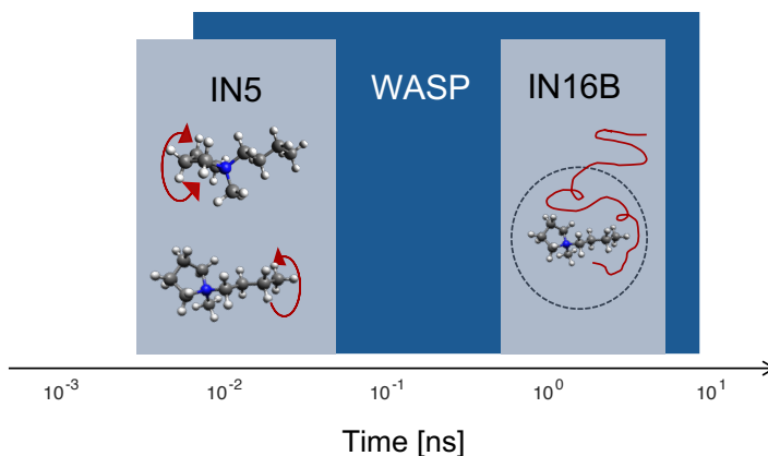
Figure 6.5: Time scales covered by the QENS instrument IN5, IN16B and WASP and examples of motions that typically occur on these time scales.
