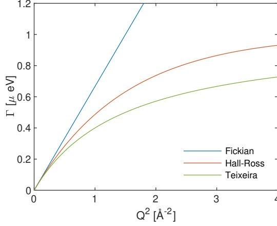
Figure 5.16: \Gamma as a function of Q^2 for different diffusion models, where \langle l^2 \rangle was set to 4 \text{ \AA} and \tau to 1 \text{ ns} for the jump diffusions and for simple diffusion D was set to 2/3 \text{ \AA}^2/\text{ns} .
