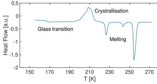
Figure 5.4: DSC trace of an ionic liquid showing a glass transition, crystallisation and melting.
