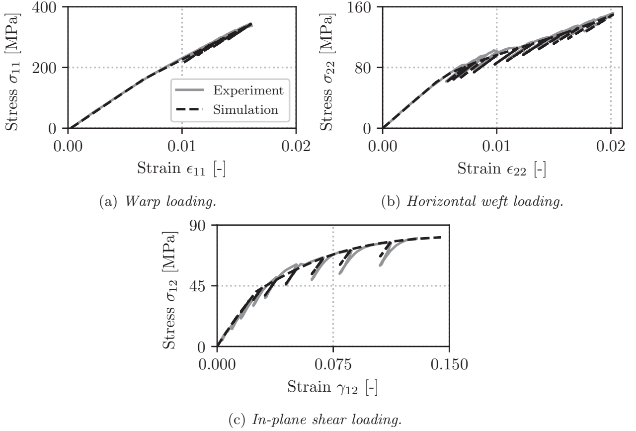
Figure 3.15: Comparison of the model predictions and experimental test results.
