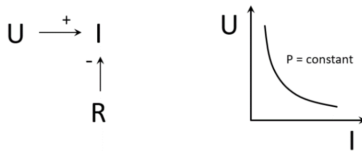
Figure 6. Ohm's law, U = R \cdot I , illustrated with a causal diagramme to the left and with a trade-off curve to the right. I = current, P = power, R = resistance, and U = voltage.
